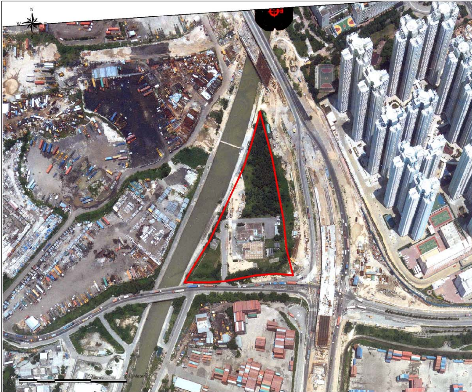
Figure 7.2 Aerial Photo of Existing Condition of the Site of the Proposed Expanded Ha Tsuen Pumping Station
