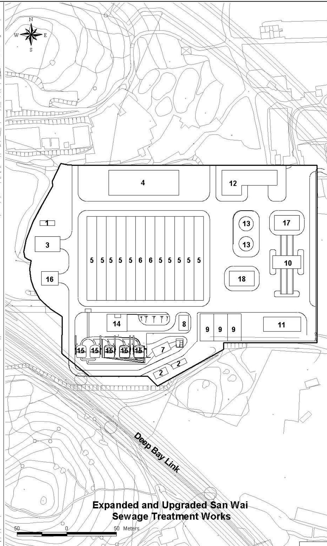
Figure A6.2 Existing and Expanded/Upgraded San Wai STW
