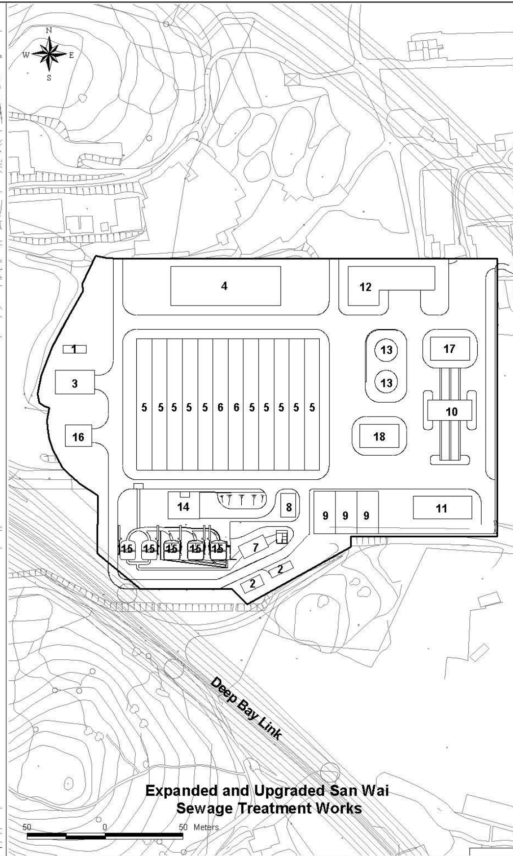
Figure 1.4 Existing and Expanded/Upgraded San Wai STW
