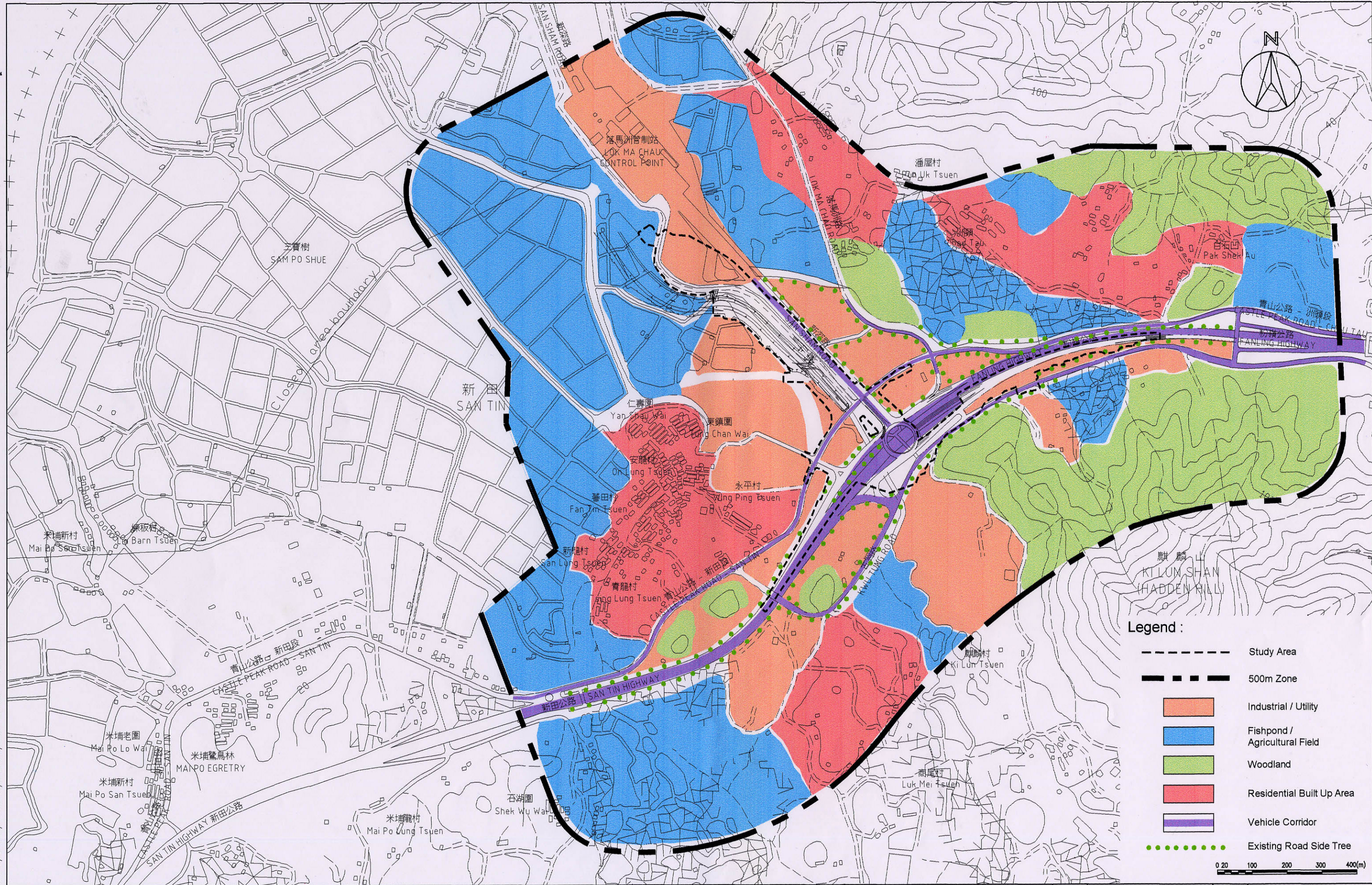
AGREEMENT No. CE 38/2002 (HY) IMPROVEMENTS TO SAN TIN INTERCHANGE - INVESTIGATION FIGURE 10.3 LANDSCAPE ELEMENTS
