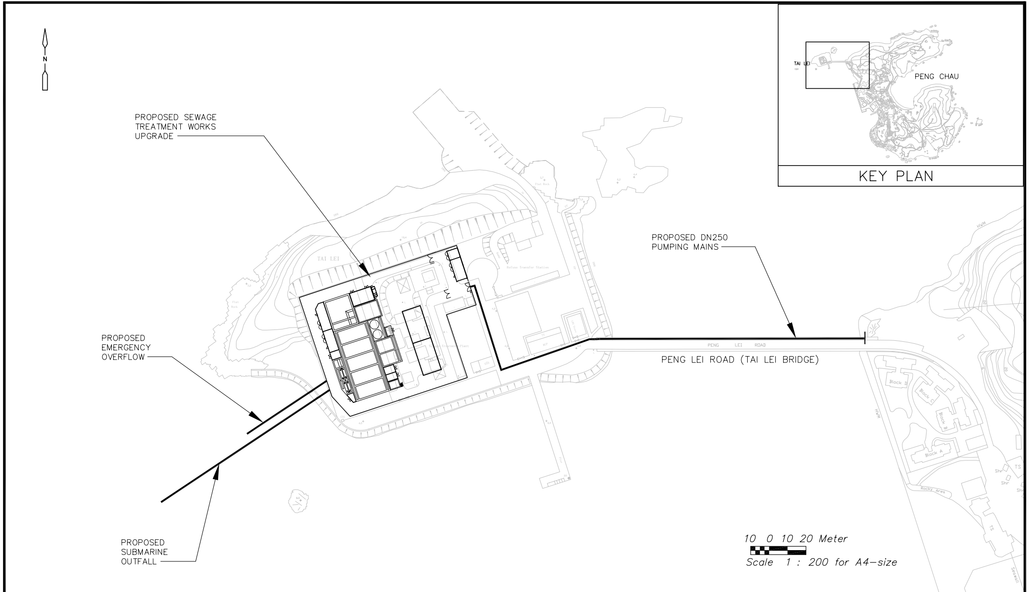
Figure 2-1 Layout plan of the Peng Chau Sewage Treatment Works Upgrade
