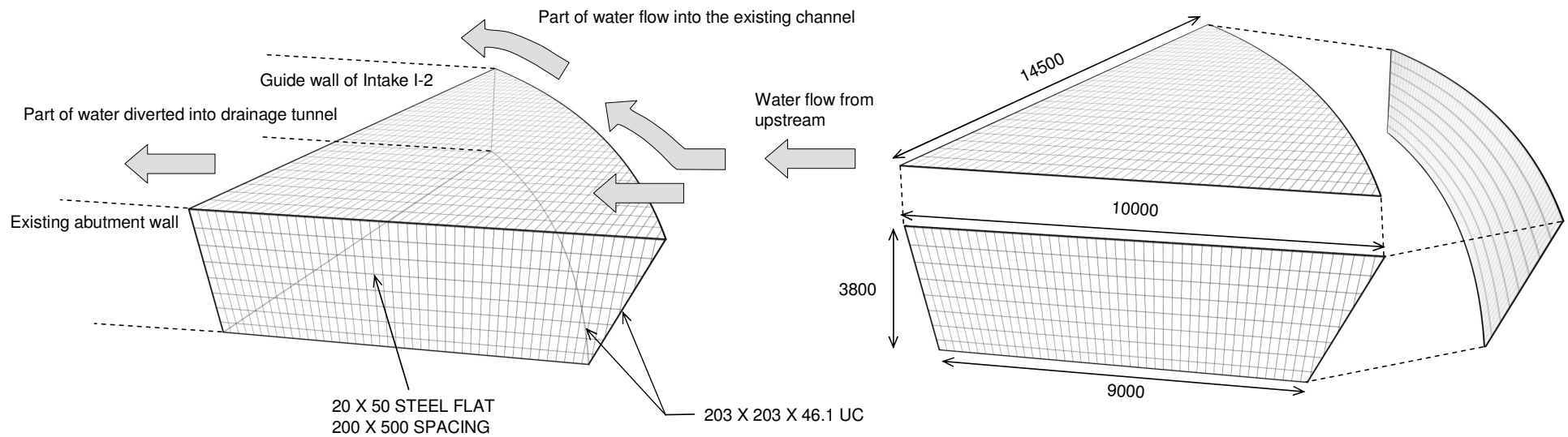
Isometric View of Trash Grill
