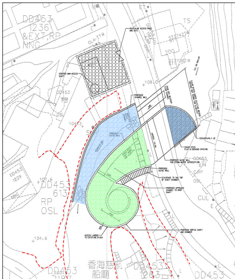
Revised Arrangement
