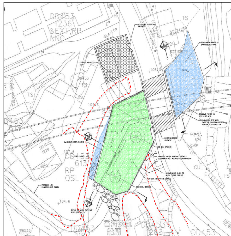
Original Arrangement
