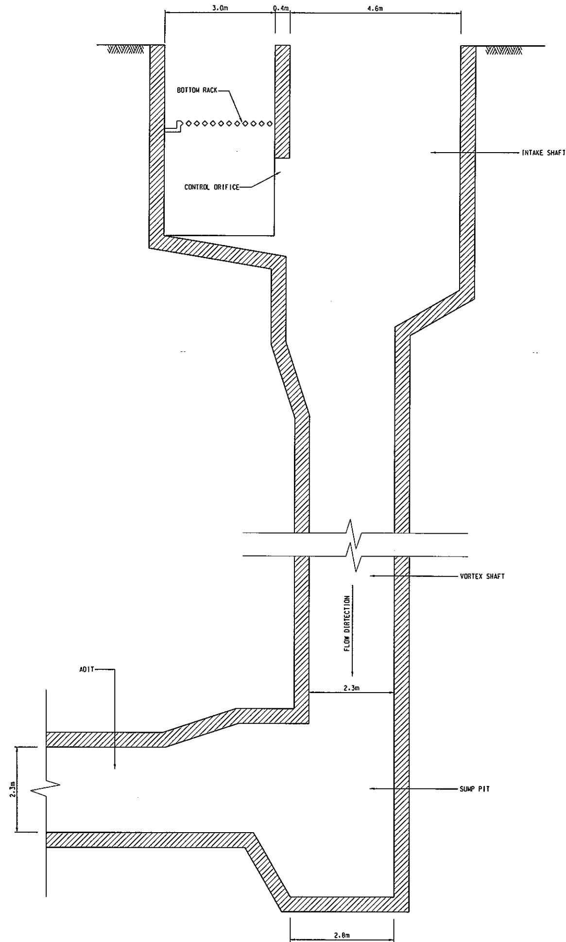
ELEVATION OF ADIT AND INTAKE/VORTEX SHAFT SCALE = 1:100 (A3)
