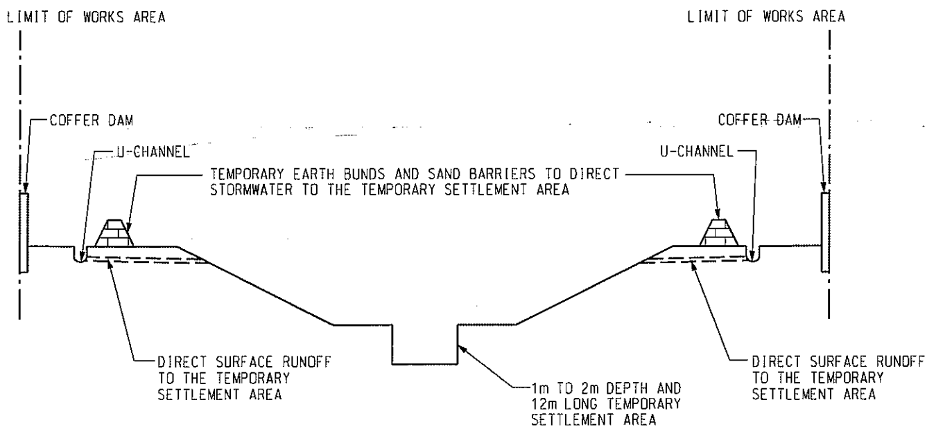
TYPICAL SECTION OF SEDIMENTATION AREA
