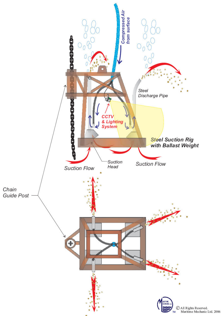
Figure 3-18 The Design of Airlift Suction Dredge Rig
