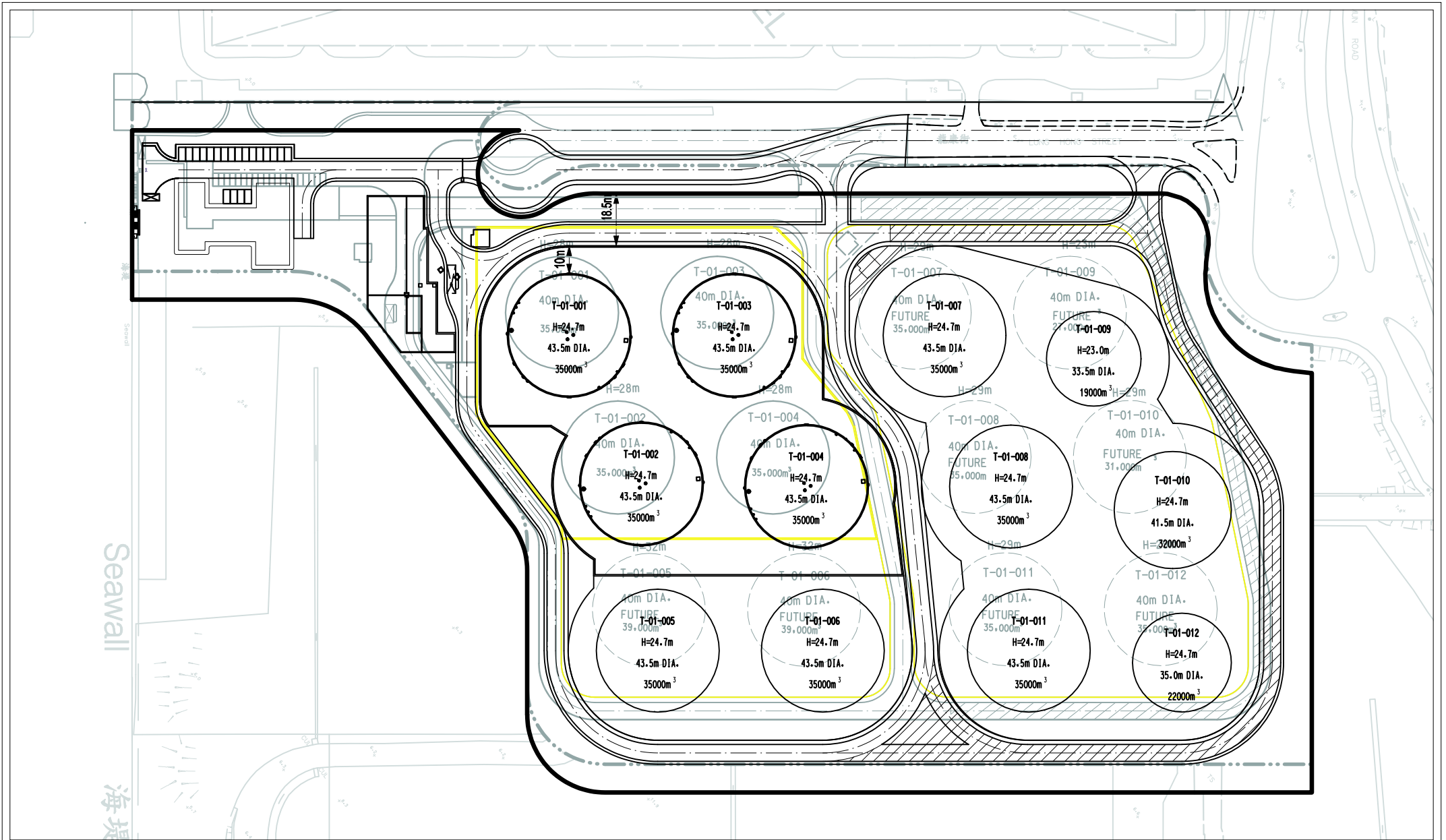
Layout of Permanent Aviation Fuel Facility Tank Farm for Variation to Environmental Permit
