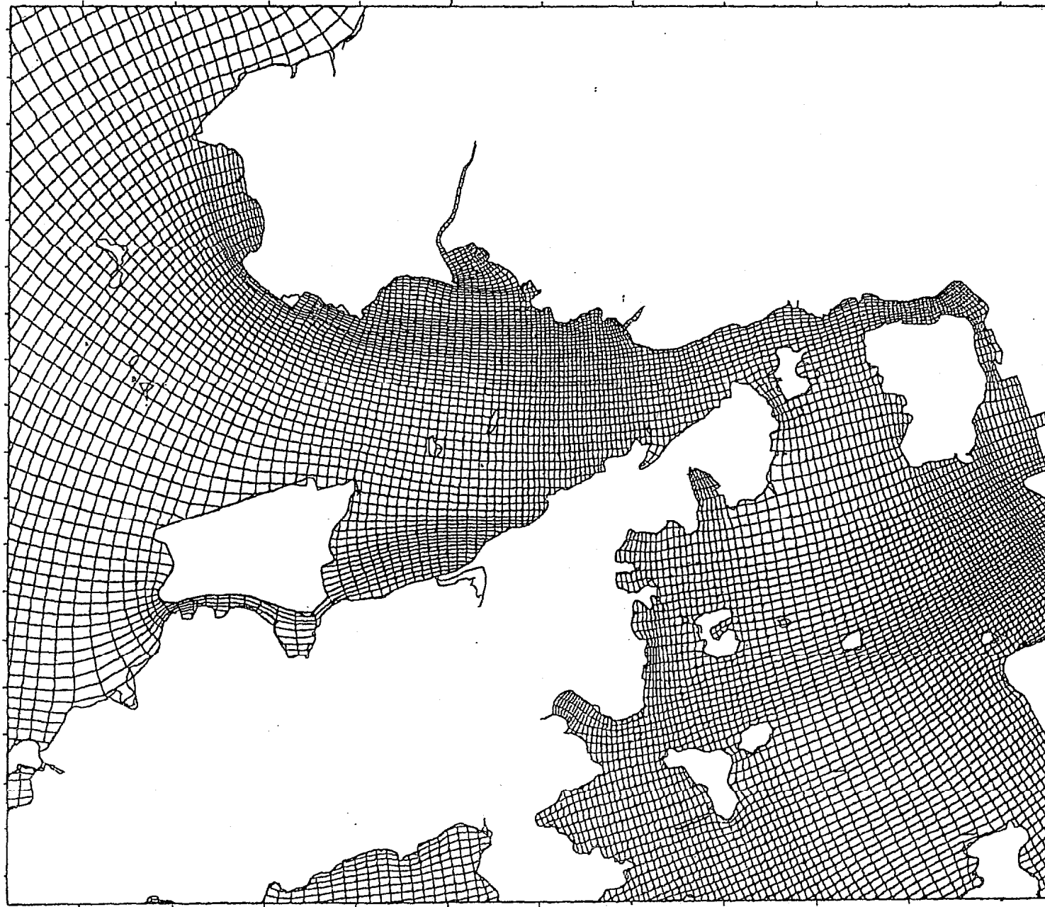
DETAIL OF THE WESTERN HARBOUR MODEL MESH
