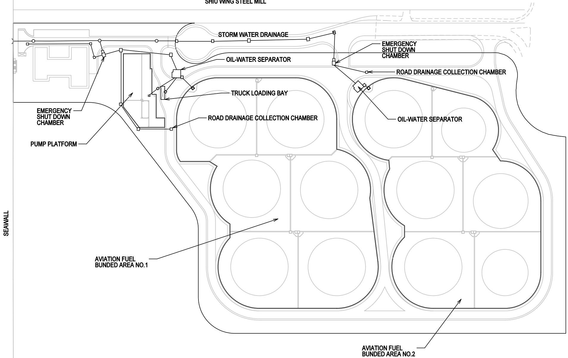
Layout Plan - Storm Water Drainage of Tankfarm and Tanks Bunded Areas
