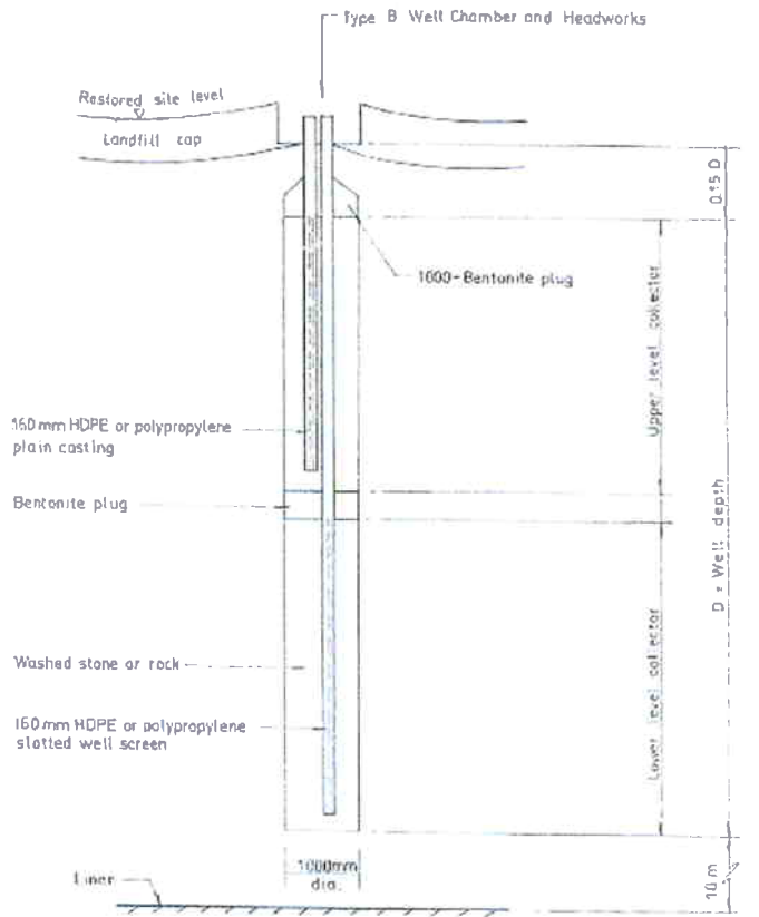
Well head & pipeline for extraction and conveyance of LFG
