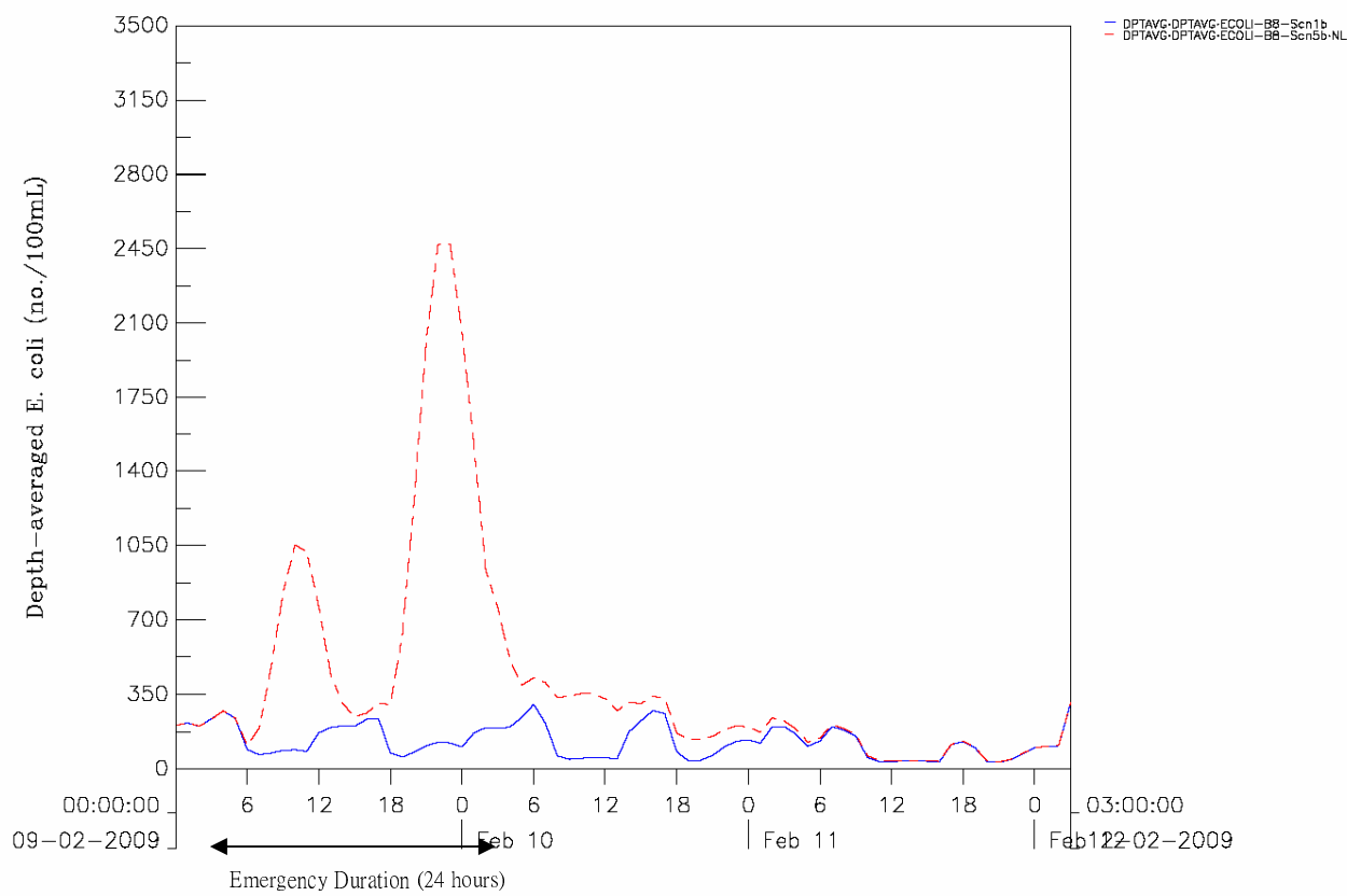
Depth-averaged E. coli Concentration under Year 2009 at Gemini Beaches (B8) Top: Scenario 5a (6Hr Emergency); Bottom: Scenario 5b (24Hr Emergency) Blue: Normal Operation; Dashed Red: Emergency Condition Figure 2 2009 Dry Season Scenario 5 (Neap Tide) Maunsell /WQ/2009/Dry/plot Scn5-2009-Dry-NL.ssn
