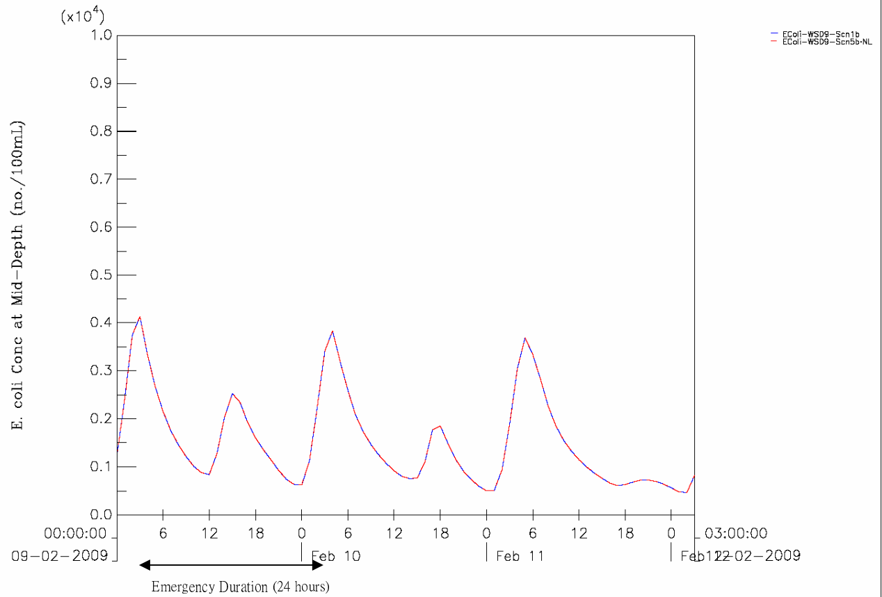
E. coli Concentration at Mid-depth under Year 2009 at WSD9 Top: Scenario 5a (6Hr Emergency); Bottom: Scenario 5b (24Hr Emergency) Blue: Normal Operation; Dashed Red: Emergency Condition
