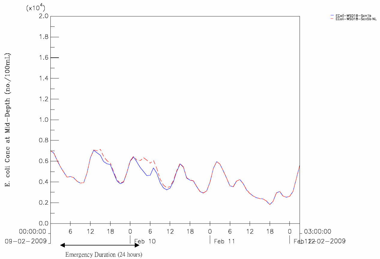
E. coli Concentration at Mid-depth under Year 2009 at WSD18 Top: Scenario 5a (6Hr Emergency); Bottom: Scenario 5b (24Hr Emergency) Blue: Normal Operation; Dashed Red: Emergency Condition
