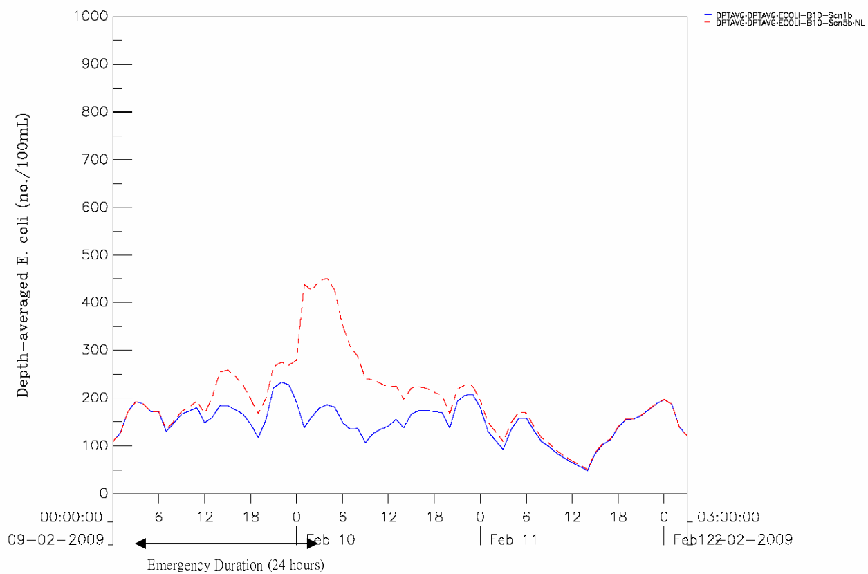
Depth-averaged E. coli Concentration under Year 2009 at Casam Beach (B10) Top: Scenario 5a (6Hr Emergency); Bottom: Scenario 5b (24Hr Emergency) Blue: Normal Operation; Dashed Red: Emergency Condition
