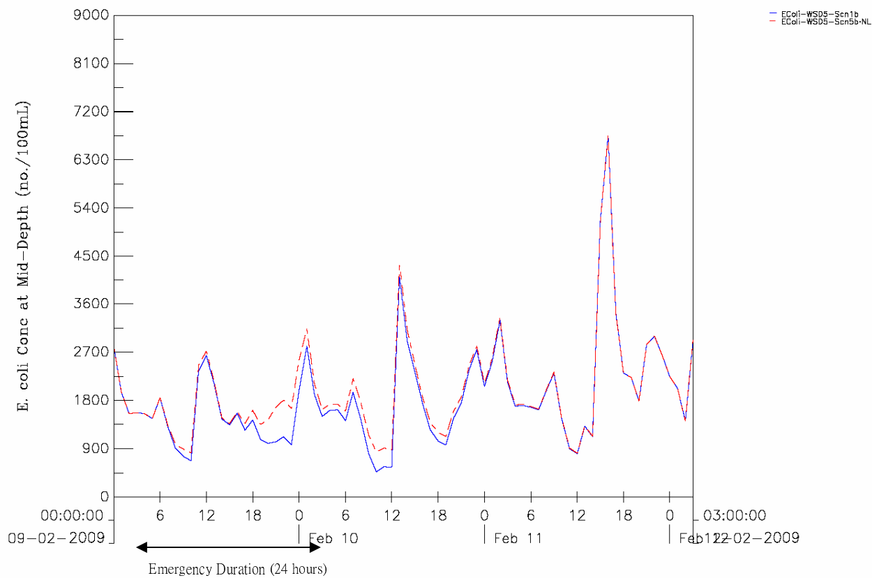
E. coli Concentration at Mid-depth under Year 2009 at WSD5 Top: Scenario 5a (6Hr Emergency); Bottom: Scenario 5b (24Hr Emergency) Blue: Normal Operation; Dashed Red: Emergency Condition
