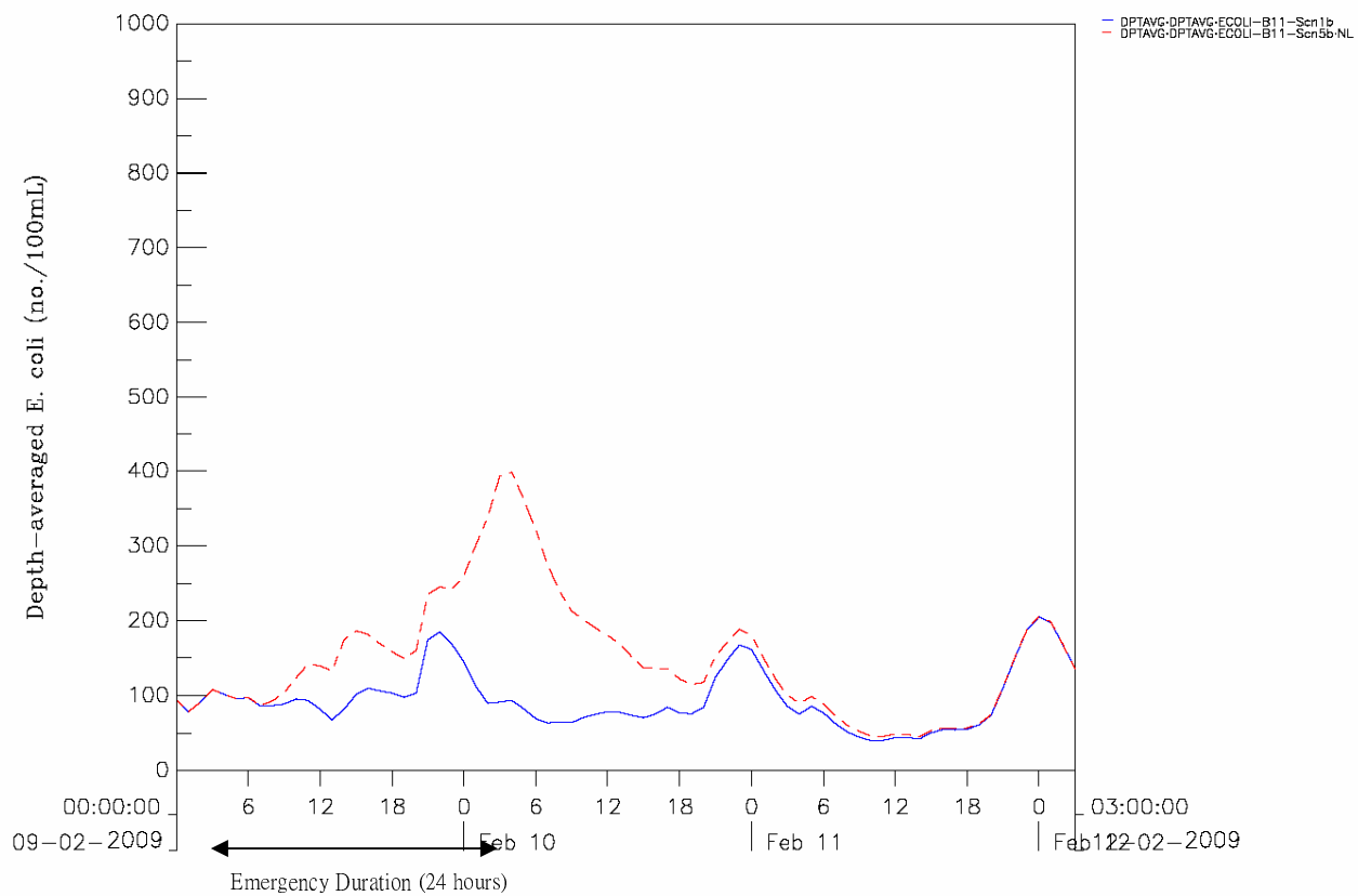
Depth-averaged E. coli Concentration under Year 2009 at Lido Beach (B11) Top: Scenario 5a (6Hr Emergency); Bottom: Scenario 5b (24Hr Emergency) Blue: Normal Operation; Dashed Red: Emergency Condition Figure 5 2009 Dry Season Scenario 5 (Neap Tide) Maunsell /WQ/2009/Dry/plot Scn5-2009-Dry-NL.ssn
