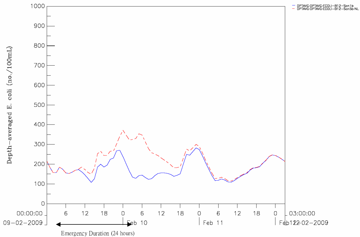
Depth-averaged E. coli Concentration under Year 2009 at Ting Kau Beach (B12) Top: Scenario 5a (6Hr Emergency); Bottom: Scenario 5b (24Hr Emergency) Blue: Normal Operation; Dashed Red: Emergency Condition Figure 6 2009 Dry Season Scenario 5 (Neap Tide) Maunsell /WQ/2009/Dry/plot Scn5-2009-Dry-NL.ssn
