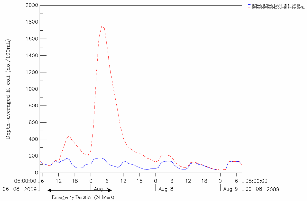
Depth-averaged E. coli Concentration under Year 2009 at Ma Wan (B14) Top: Scenario 5a (6Hr Emergency); Bottom: Scenario 5b (24Hr Emergency) Blue: Normal Operation; Dashed Red: Emergency Condition Figure 8 2009 Wet Season Scenario 5 (Neap Tide) Maunsell /WQ/2009/Wet/plot Scn5-2009-Wet-NL.ssn
