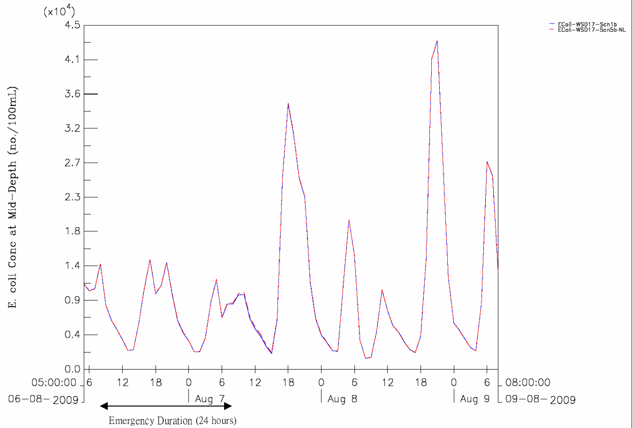
E. coli Concentration at Mid-depth under Year 2009 at WSD17 Top: Scenario 5a (6Hr Emergency); Bottom: Scenario 5b (24Hr Emergency) Blue: Normal Operation; Dashed Red: Emergency Condition Figure 15 2009 Wet Season Scenario 5 (Neap Tide) Maunsell /WQ/2009/Wet/plot Scn5-2009-Wet-NL.ssn
