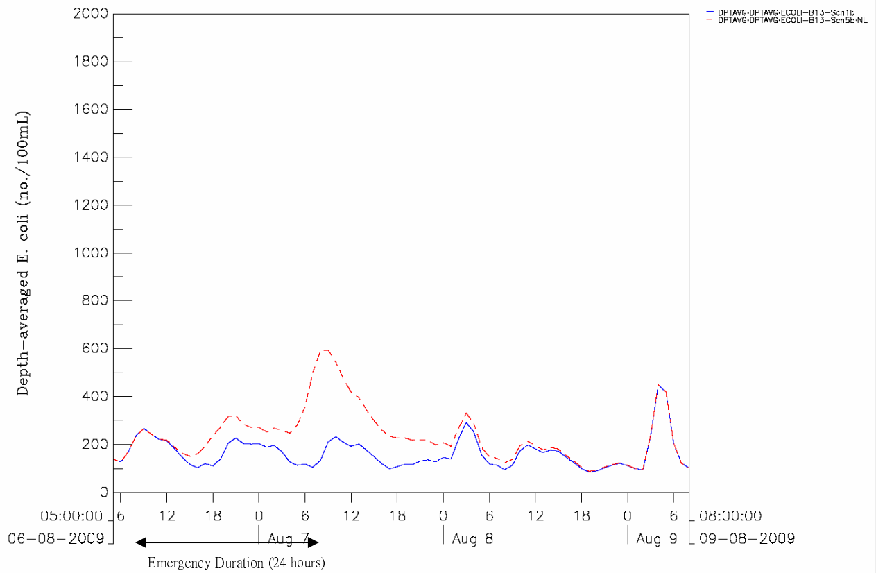
Depth-averaged E. coli Concentration under Year 2009 at Approach Beach (B13) Top: Scenario 5a (6Hr Emergency); Bottom: Scenario 5b (24Hr Emergency) Blue: Normal Operation; Dashed Red: Emergency Condition Figure 7 2009 Wet Season Scenario 5 (Neap Tide) Maunsell /WQ/2009/Wet/plot Scn5-2009-Wet-NL.ssn
