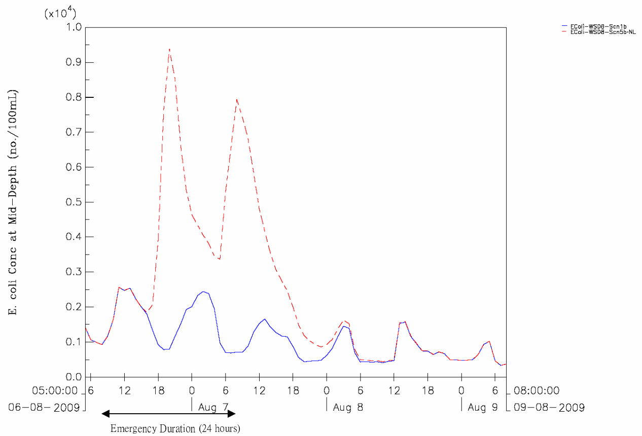
E. coli Concentration at Mid-depth under Year 2009 at WSD8 Top: Scenario 5a (6Hr Emergency); Bottom: Scenario 5b (24Hr Emergency) Blue: Normal Operation; Dashed Red: Emergency Condition
