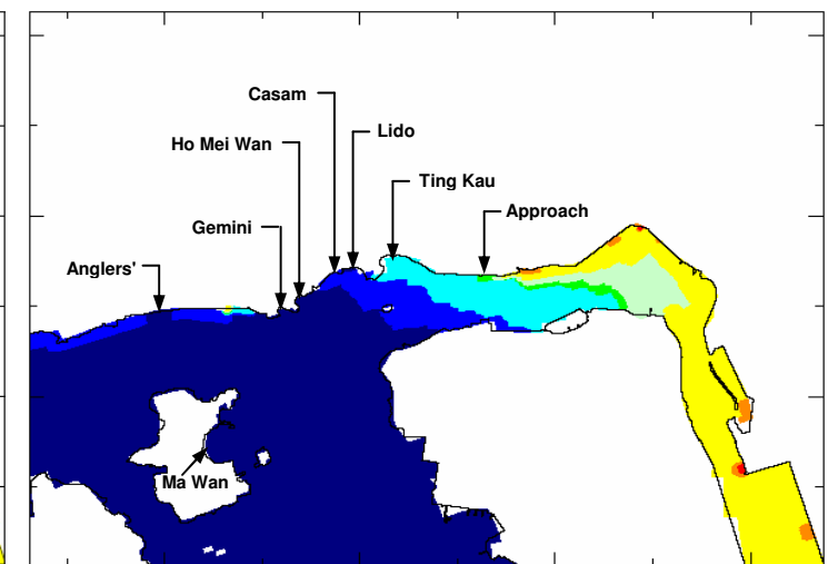
Ultimate Year HATS Stage 2B with Disinfection
