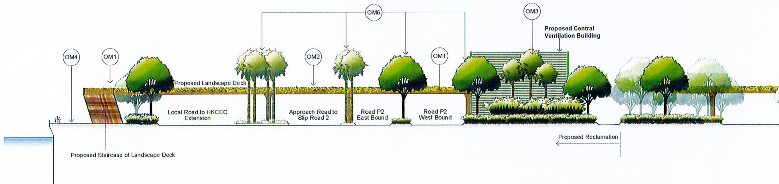
Section B-B
