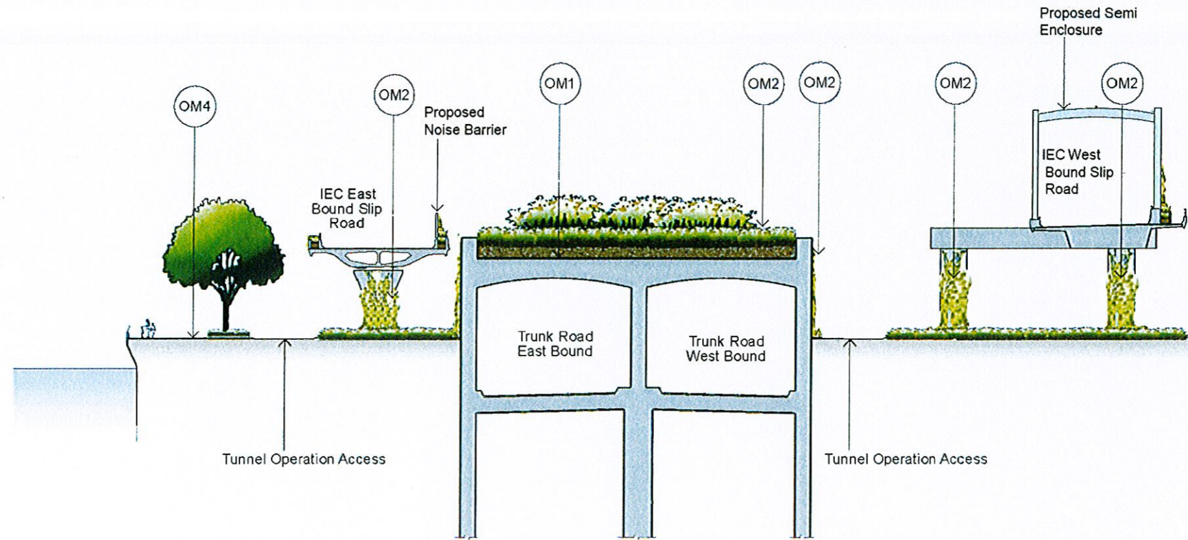
Section I-I
