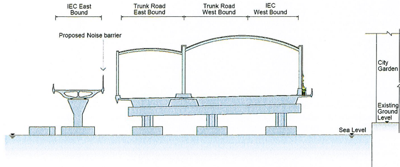
Section J-J
