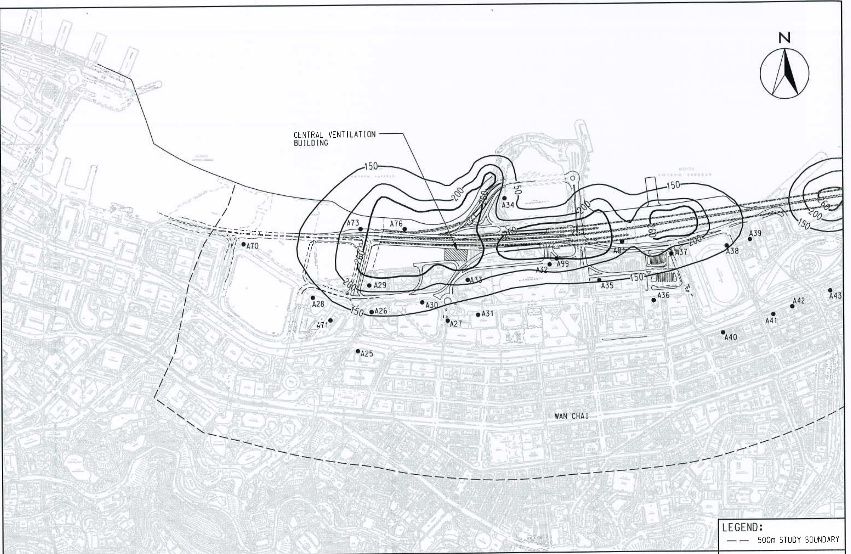
WAN CHAI DEVELOPMENT PHASE II - PLANNING AND ENGINEERING REVIEW CONTOURS OF CUMULATIVE MAXIMUM 24-HOUR TSP CONCENTRATION IN \mu\text{g}/\text{m}^3 AT 1.5m ABOVE GROUND (WAN CHAI SECTION) (SCENARIO 3)
