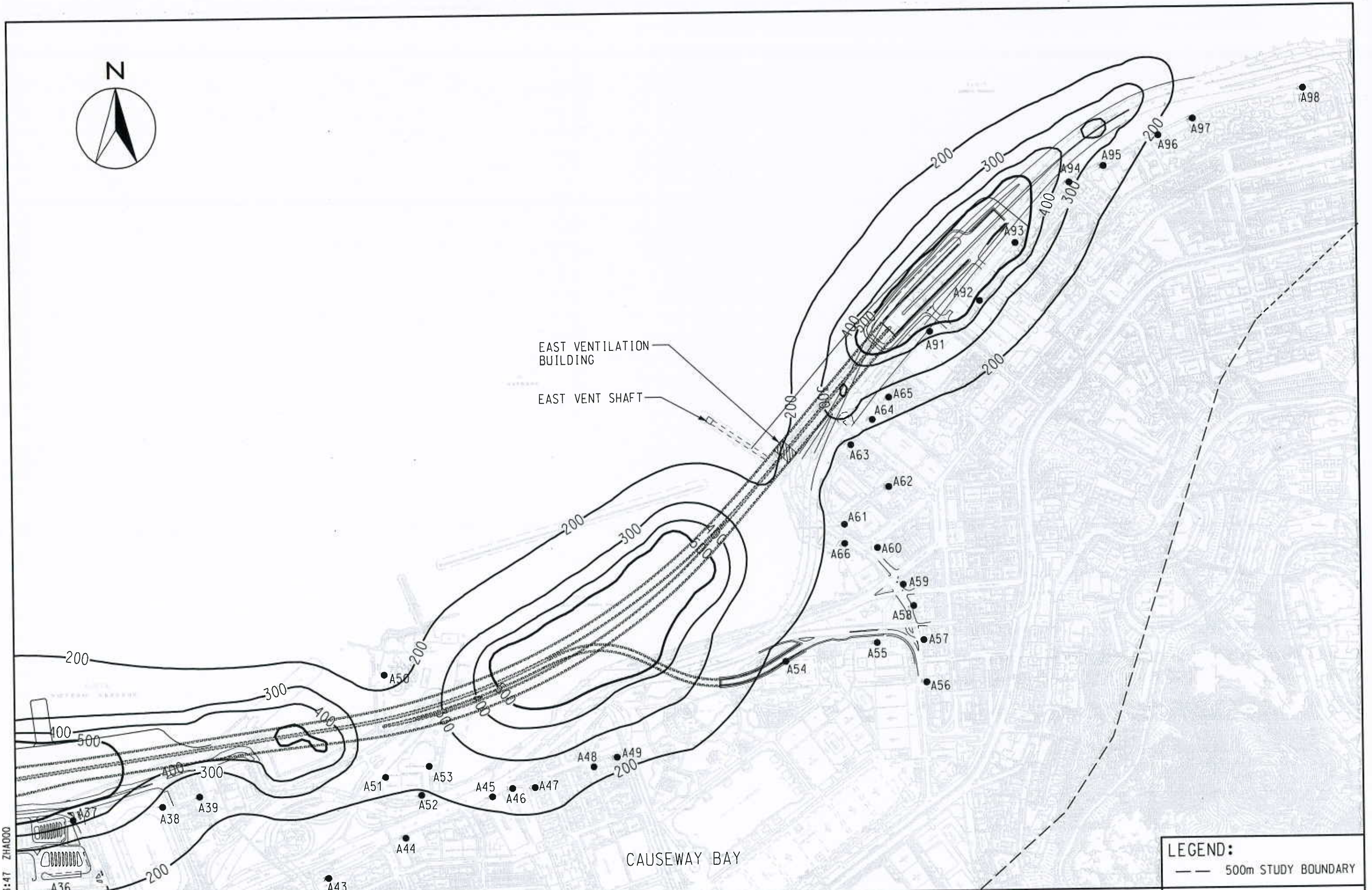
WAN CHAI DEVELOPMENT PHASE II - PLANNING AND ENGINEERING REVIEW CONTOURS OF CUMULATIVE MAXIMUM 1-HOUR TSP CONCENTRATION IN \mu\text{g}/\text{m}^3 AT 1.5m ABOVE GROUND (CAUSEWAY BAY & IECL SECTION) (SCENARIO 4)
