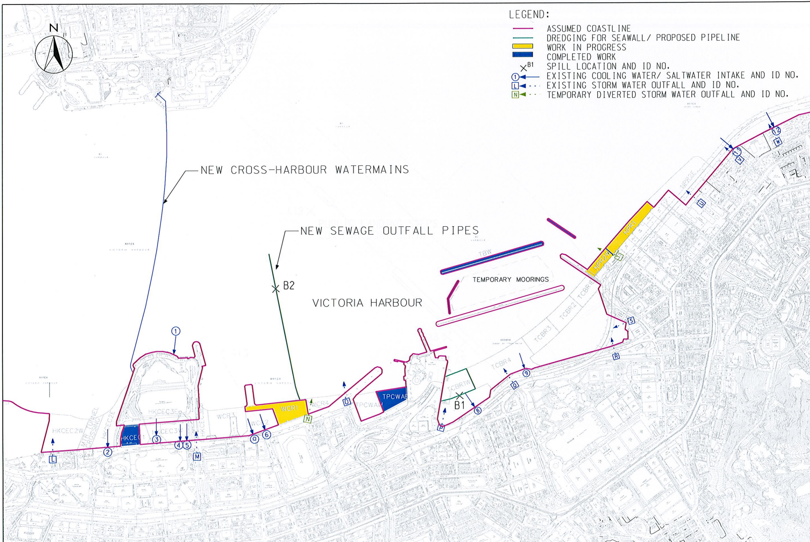
MAUNSELL | AECOM Maunsell Consultants Asia Ltd WAN CHAI DEVELOPMENT PHASE II - PLANNING AND ENGINEERING REVIEW CONSTRUCTION PHASE MODELLING SCENARIO 2B FIGURE 5.8
