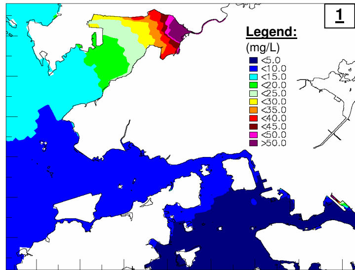
Scenario 2b (Assumed SS Level in the PPSTW Effluent: 120mg/L)
