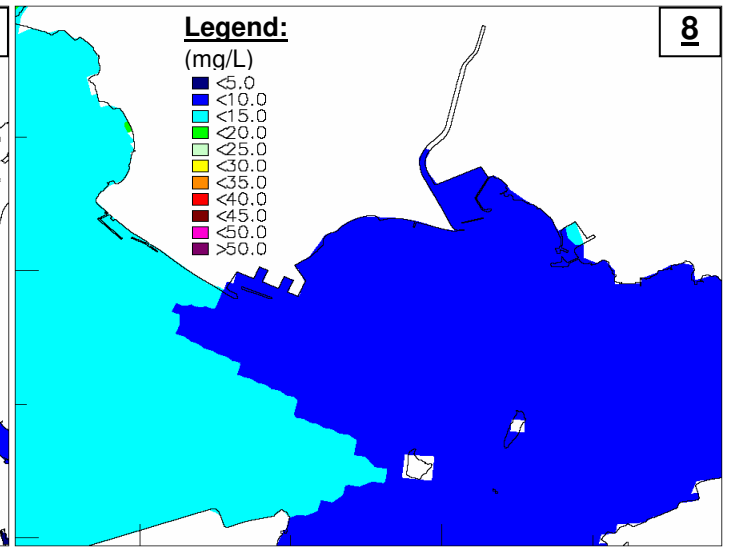
Scenario 2c (Assumed SS Level in the PPSTW Effluent: 30mg/L)
