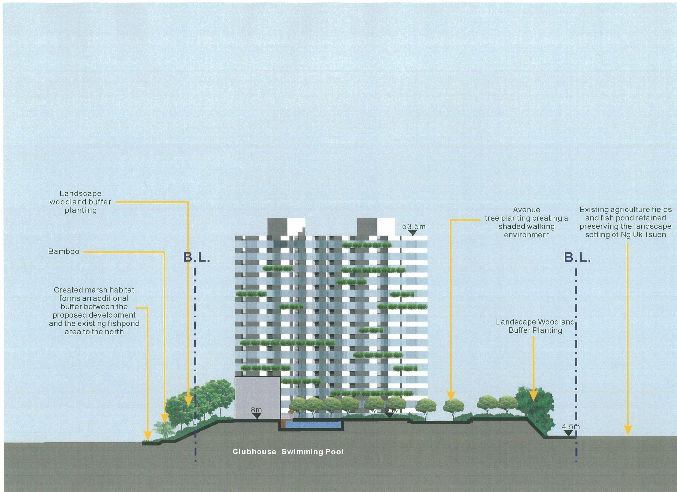
Section B-B'
