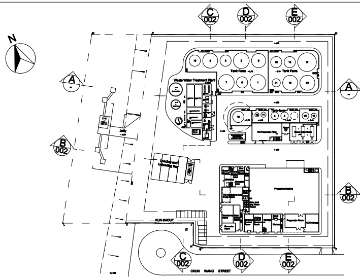
MASTER LAYOUT PLAN
