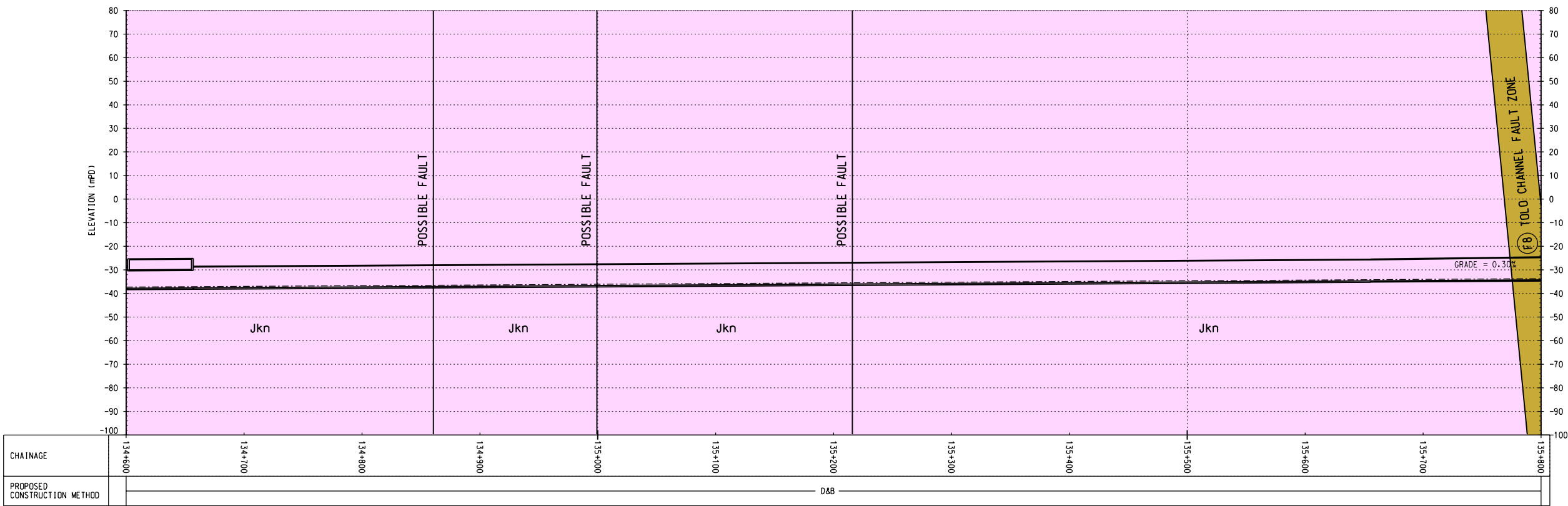
PROFILE SCALE 1:4000 HORI. 1:2000 VERT.
