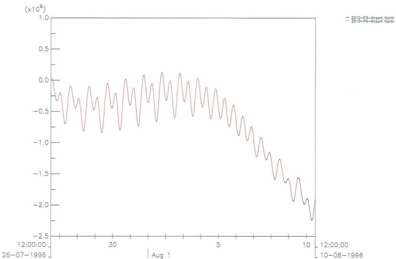
2010 (Baseline) – 3rd Production (P3) and 4th Production (P4) Time History Plot of Accumulated and Momentary Flow at Airport North – Wet Season
