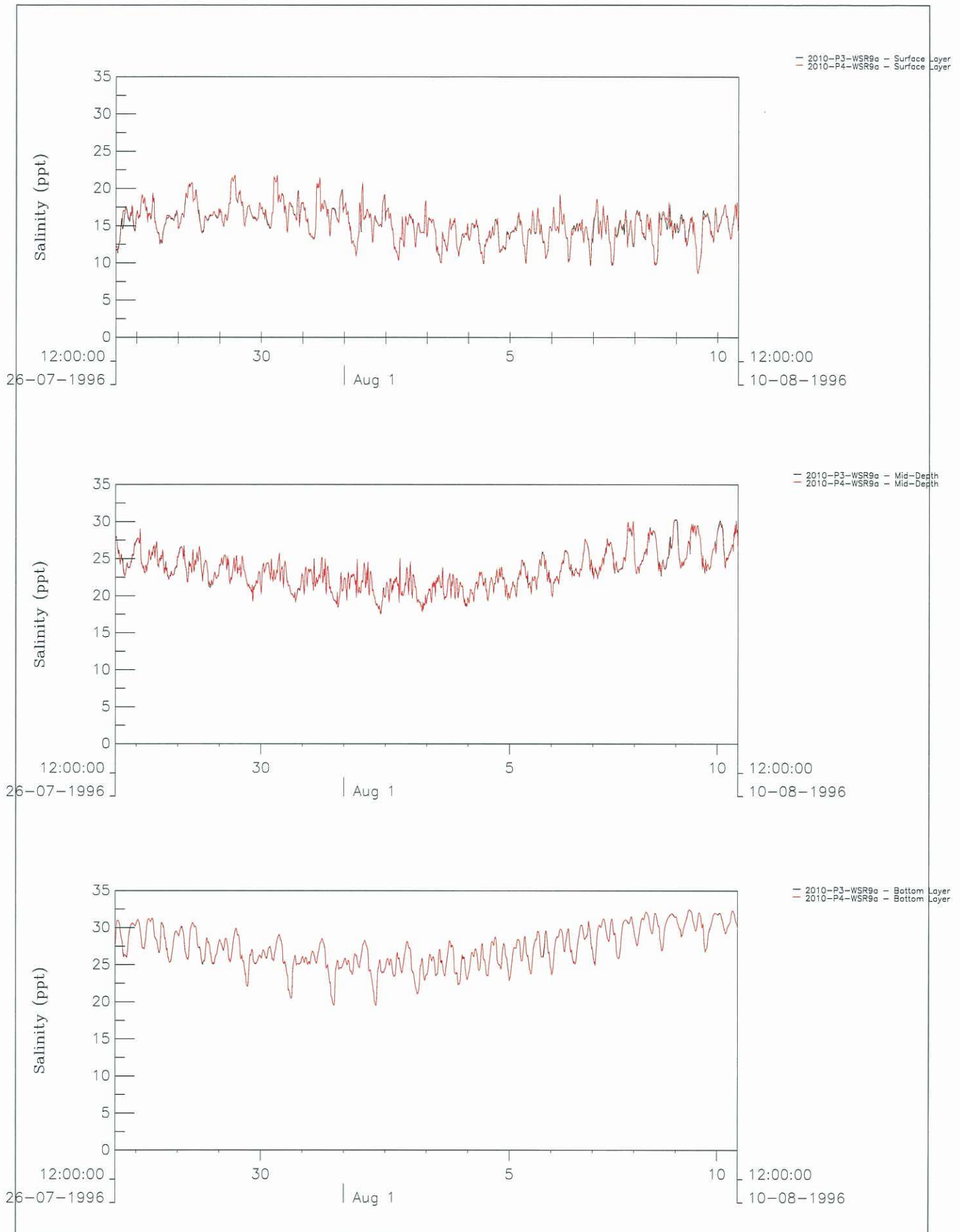
2010 (Baseline) – 3rd Production (P3) and 4th Production (P4) Time history plots of Salinity at WSR9a, Wet Season (Top: Surface Layer; Middle: Mid-Depth; Bottom: Bottom Layer)
