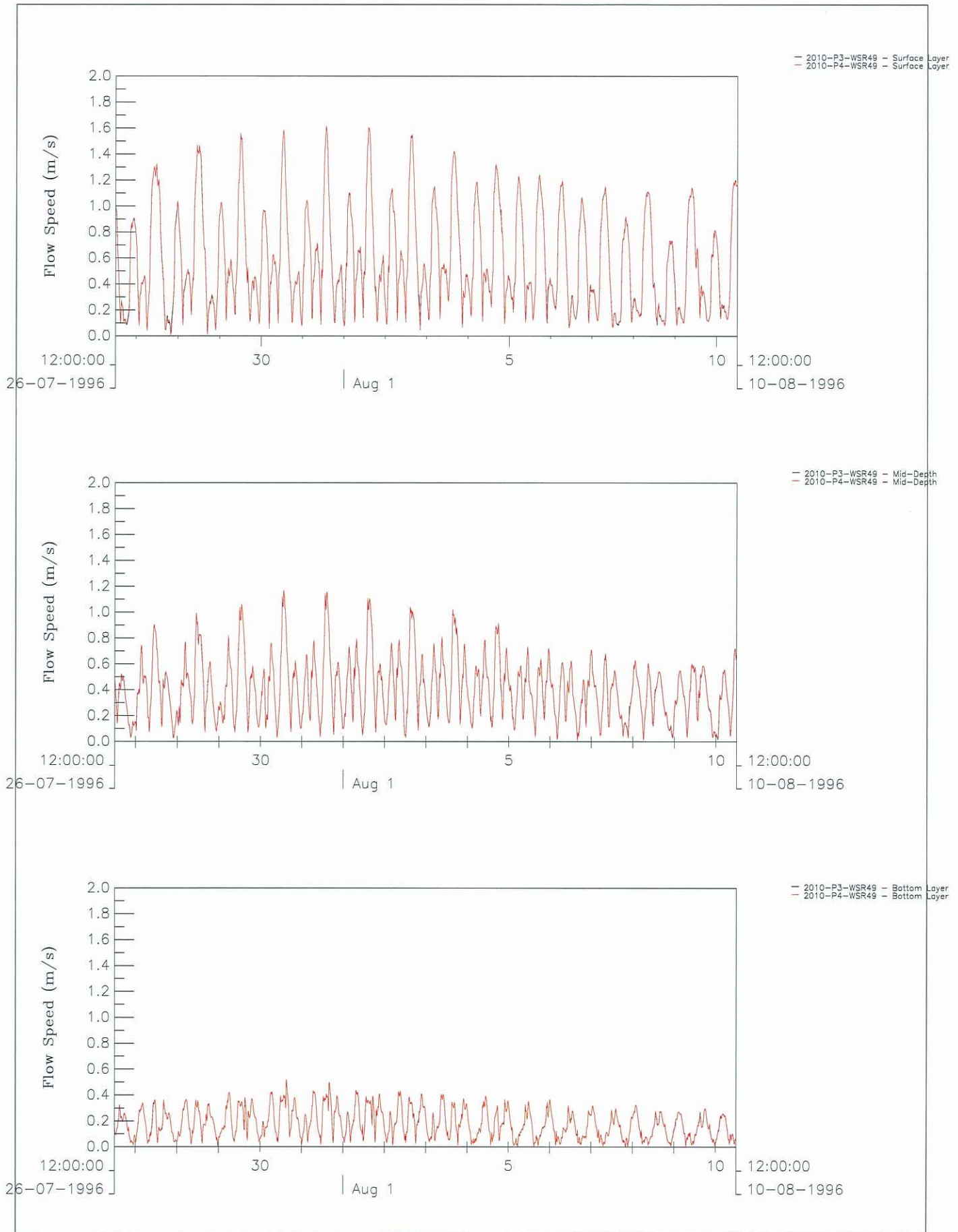
2010 (Baseline) - 3rd Production (P3) and 4th Production (P4) Time history plots of water speed at WSR49, Wet Season (Top: Surface Layer; Middle: Mid-Depth; Bottom: Bottom Layer)
