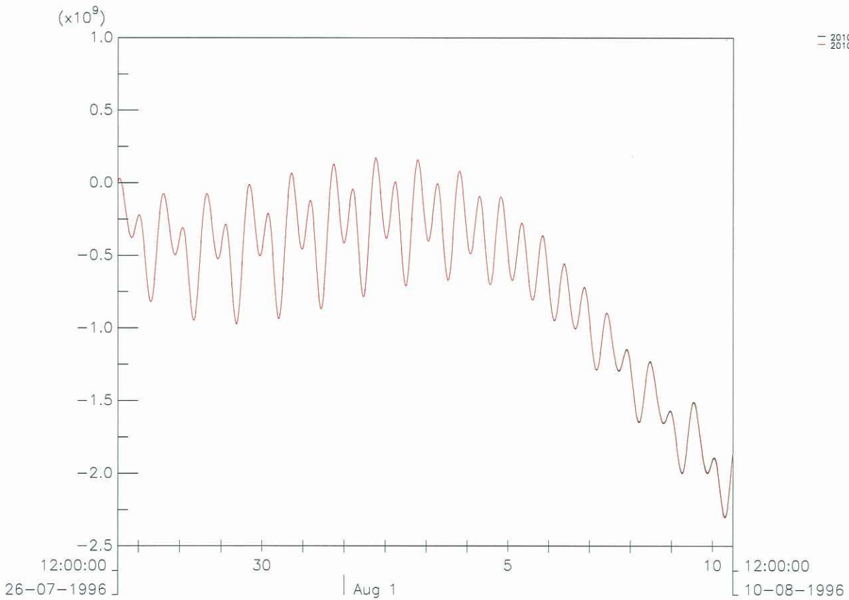
2010 (Baseline) – 3rd Production (P3) and 4th Production (P4) Time History Plot of Accumulated and Momentary Flow at Ma Wan – Wet Season
