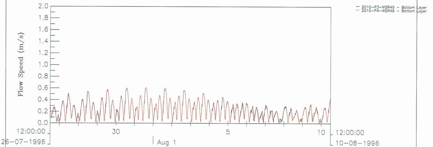
2010 (Baseline) – 3rd Production (P3) and 4th Production (P4) Time history plots of water speed at WSR49, Dry Season (Top: Surface Layer; Middle: Mid-Depth; Bottom: Bottom Layer)
