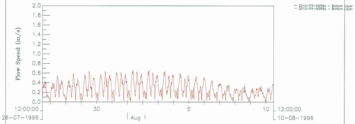
2010 (Baseline) – 3rd Production (P3) and 4th Production (P4) Time history plots of water speed at WSR9a, Wet Season (Top: Surface Layer; Middle: Mid-Depth; Bottom: Bottom Layer)
