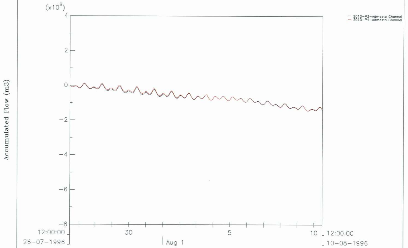
2010 (Baseline) – 3rd Production (P3) and 4th Production (P4) Time History Plot of Accumulated and Momentary Flow at Admasta Channel – Dry Season
