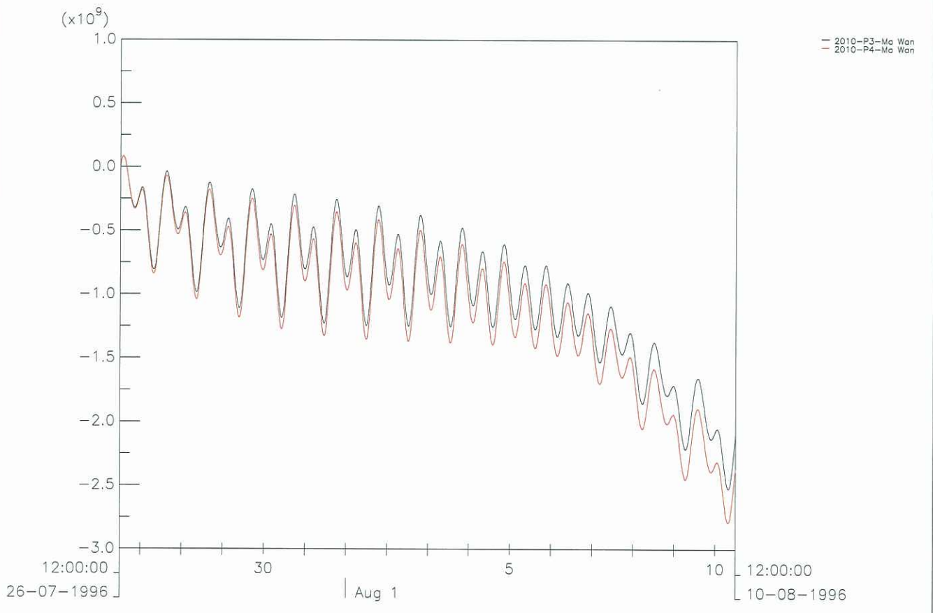
2010 (Baseline) – 3rd Production (P3) and 4th Production (P4) Time History Plot of Accumulated and Momentary Flow at Ma Wan – Dry Season
