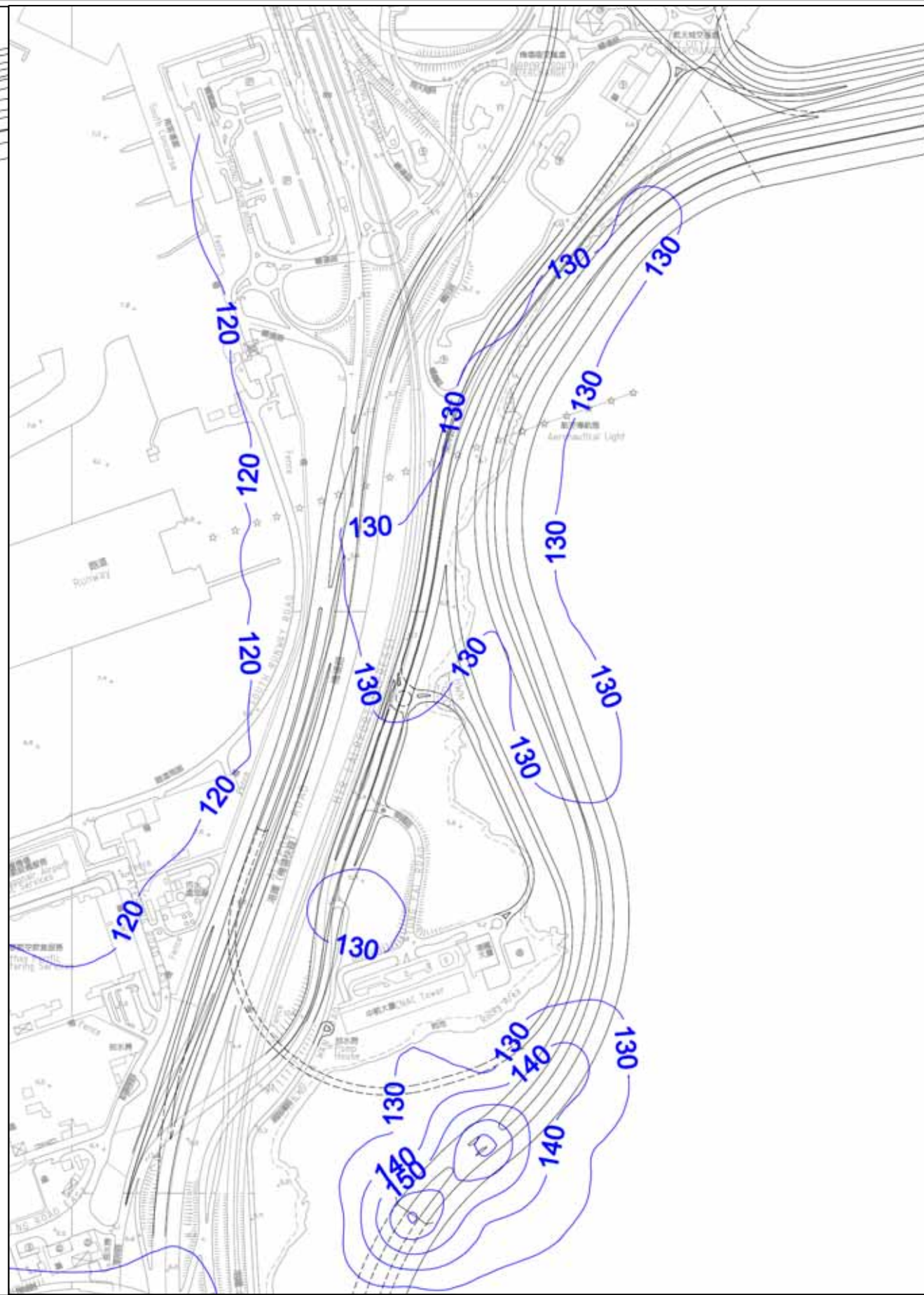
24-hr NO 2
