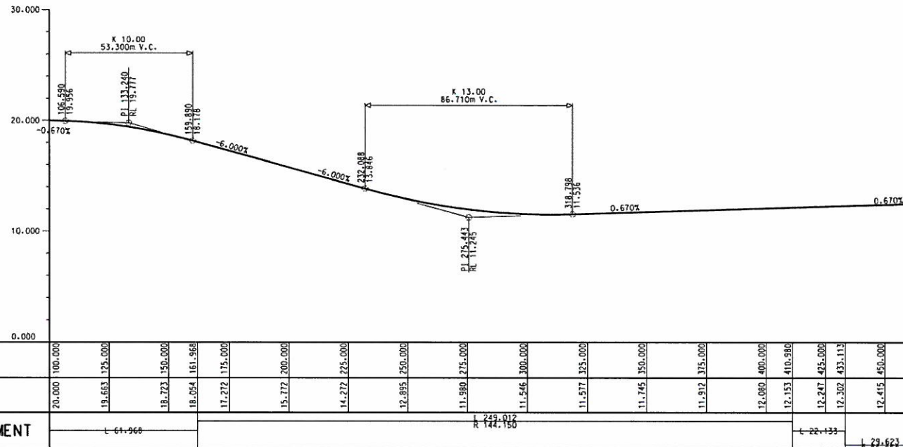
VERTICAL PROFILE A100 HORIZONTAL SCALE AT 1:1000 VERTICAL SCALE AT 1:200
