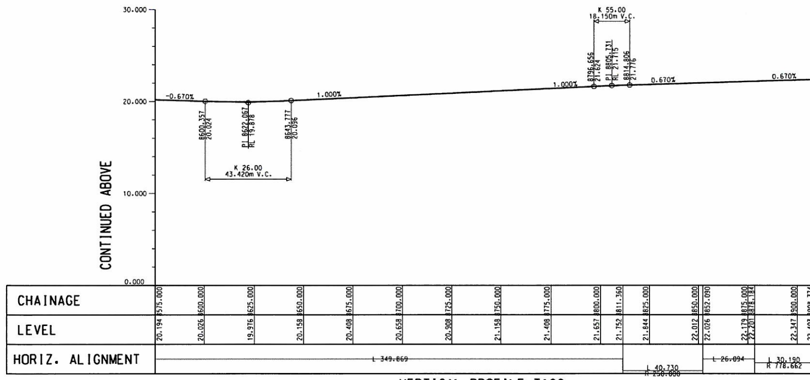
VERTICAL PROFILE T100 HORIZONTAL SCALE A1 1:1000 VERTICAL SCALE A1 1:200
