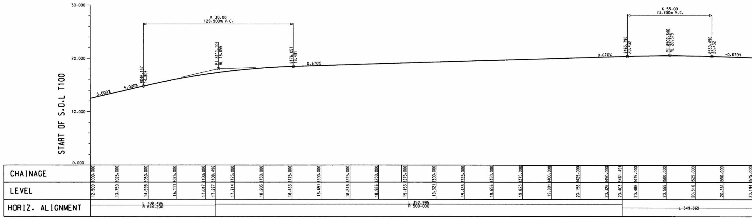
VERTICAL PROFILE T100 HORIZONTAL SCALE A1 1:1000 VERTICAL SCALE A1 1:200
