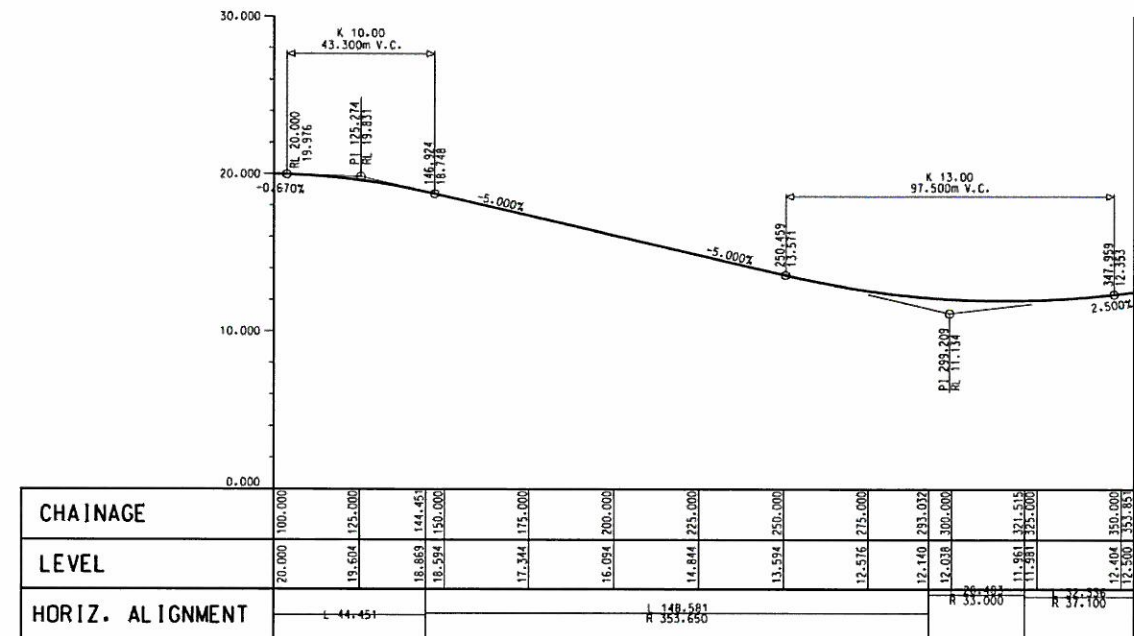
VERTICAL PROFILE A200 HORIZONTAL SCALE AT 1:1000 VERTICAL SCALE AT 1:200
