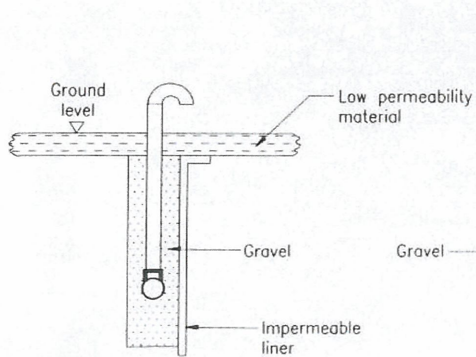
CROSS SECTION (TYP.)
