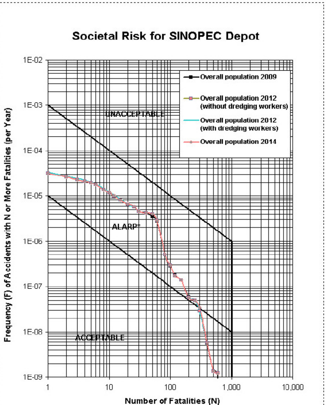
Figure 7.11 Societal Risk for SINOPEC Depot for Years 2009, 2012 and 2014
