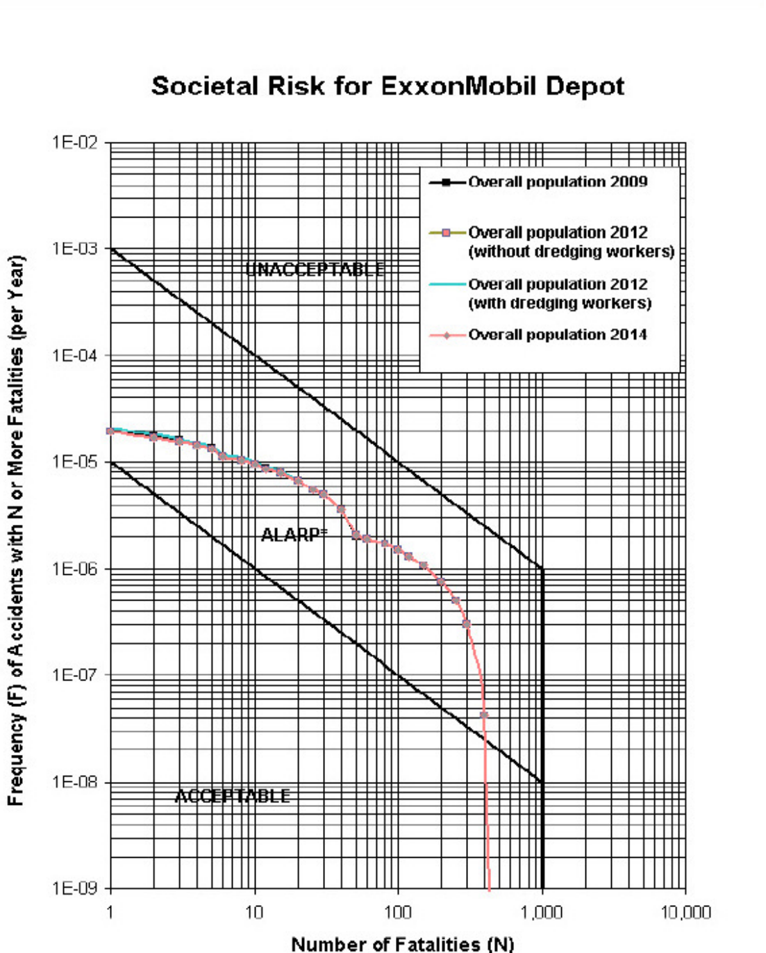
Figure 7.12 Societal Risk for ExxonMobil Depot for Years 2009, 2012 and 2014
