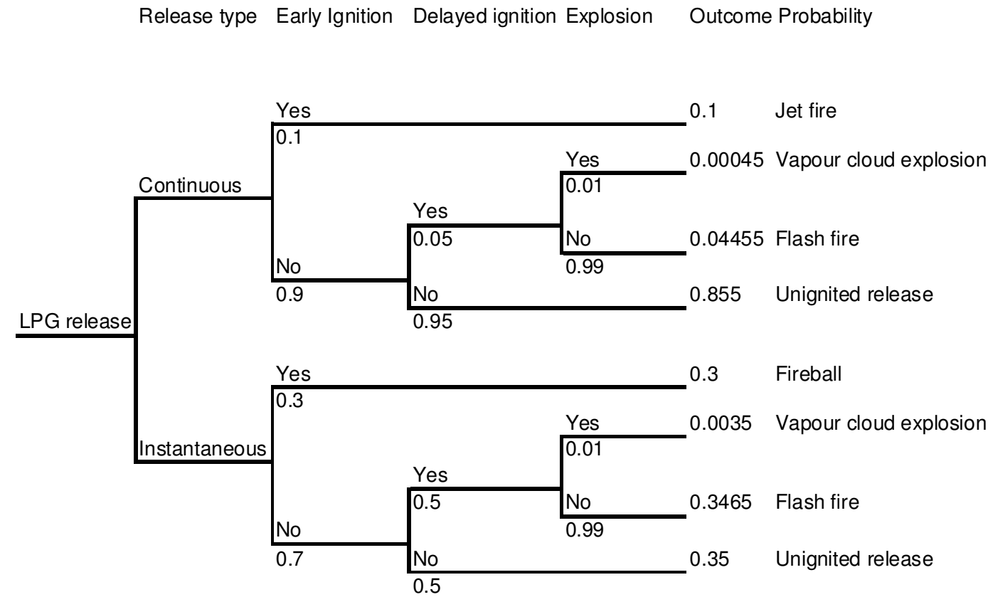
Figure 7.8 Outcome Event Tree (Above Ground LPG Storage Vessels in Exxon Mobil Depot)
