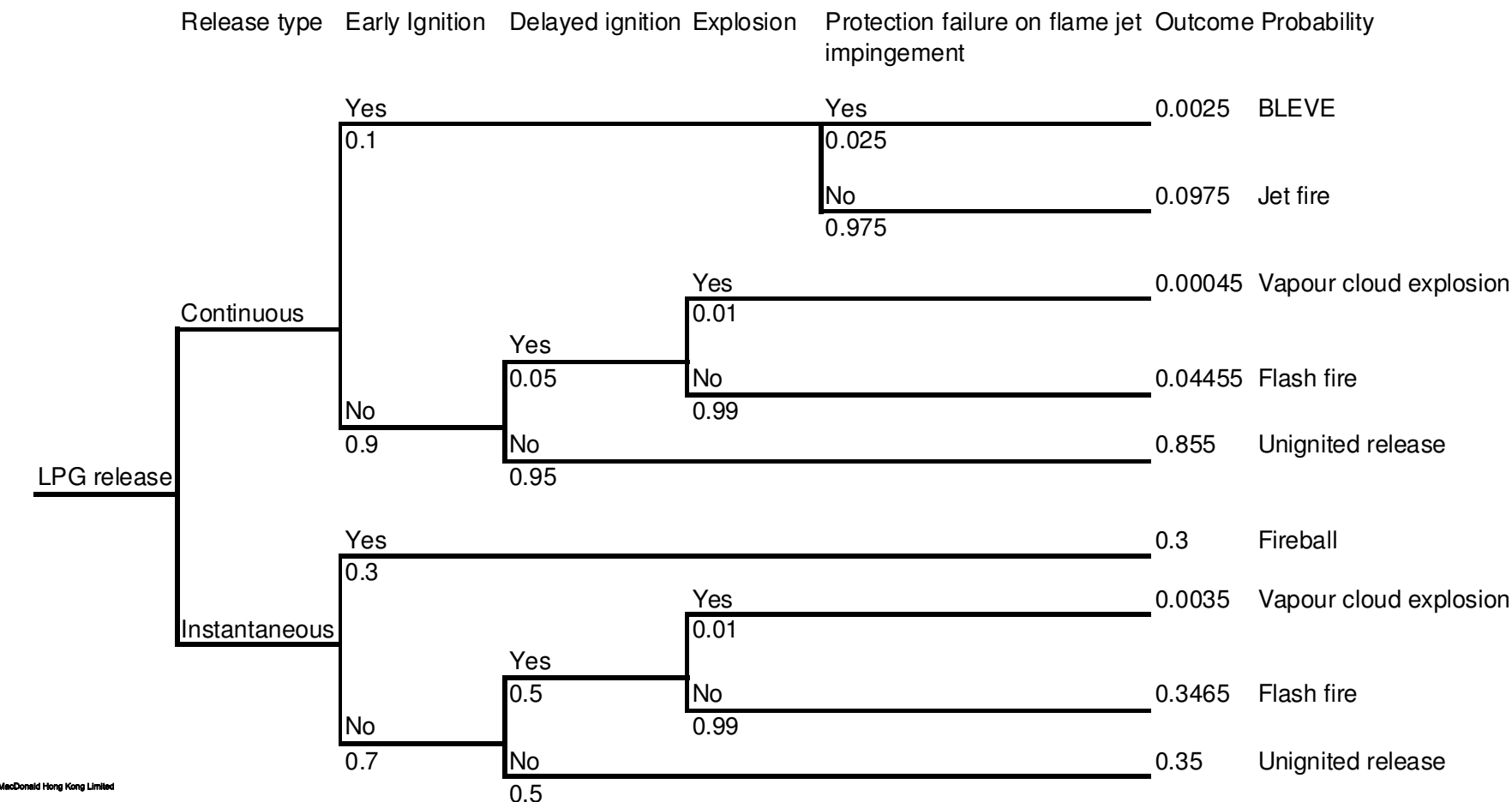
Figure 7.8 Outcome Event Tree (Above Ground LPG Storage Vessels in Exxon Mobil Depot)
