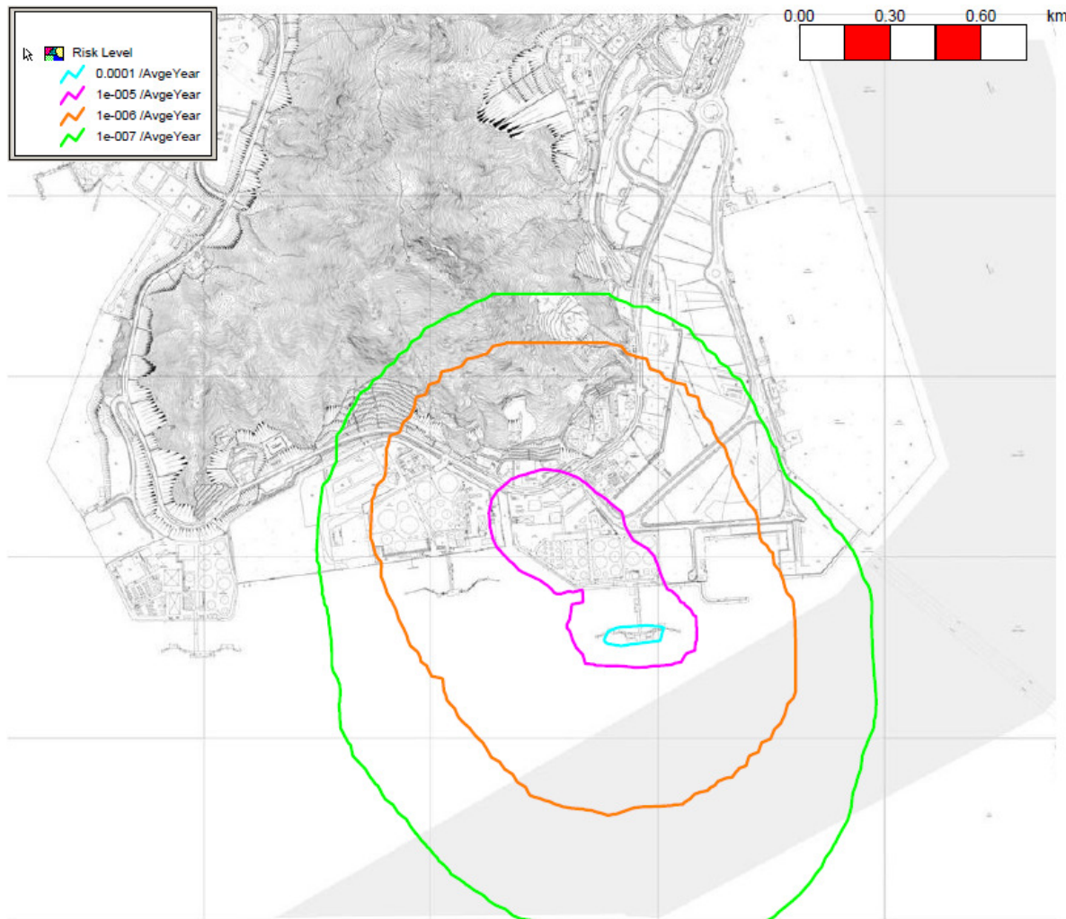
Figure 7.9 Individual Risk for SINOPEC Depot N11
