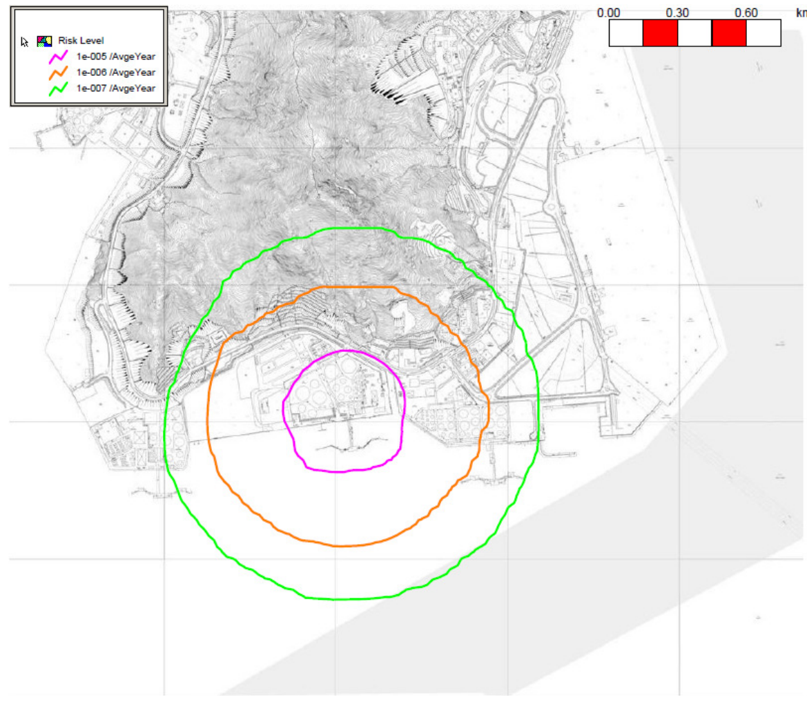
Figure 7.10 Individual Risk for ExxonMobil Depot N6
