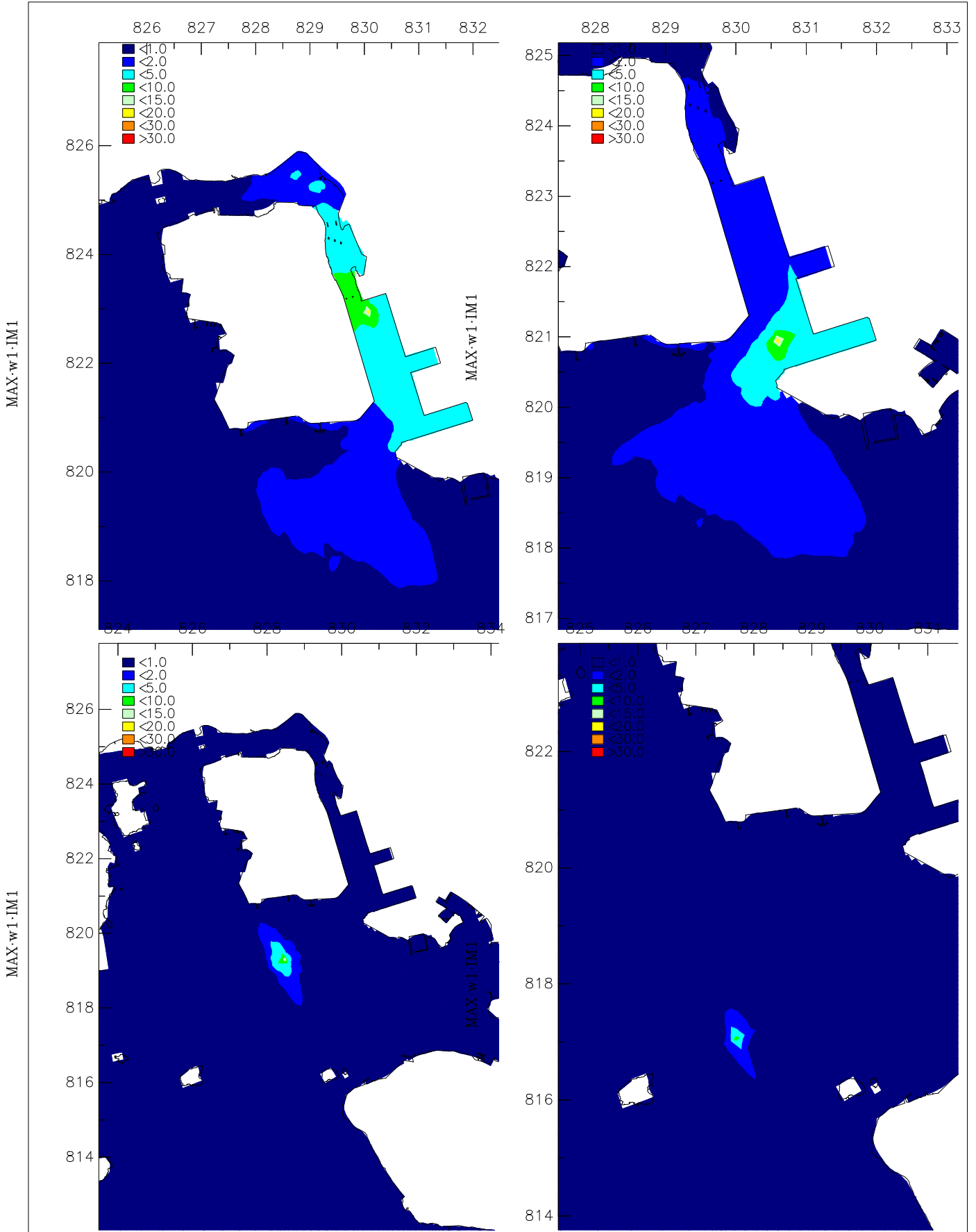
Max. Depth averaged tracer concentration (mg/L) due to different source locations
