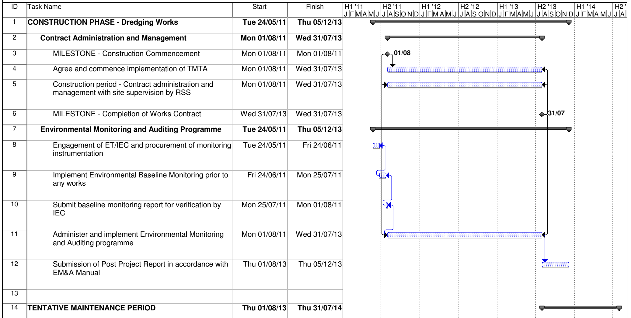
Figure 1.4 Tentative Dredging Programme (developed based on 20091210 KCTB Dredging Project Programme)
