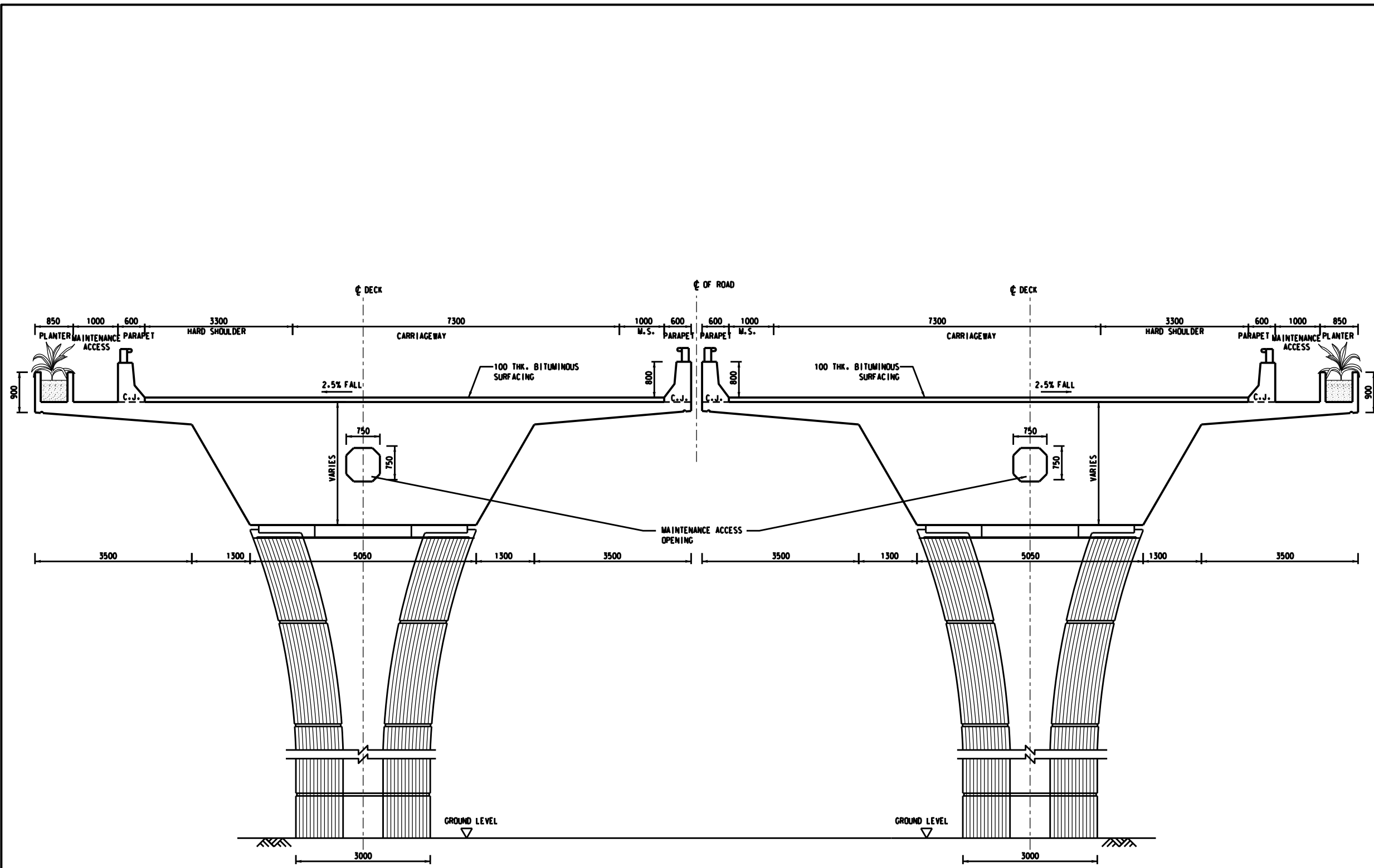
TYPICAL SECTION OF TRUNK ROAD VIADUCT AT PIER SUPPORT
