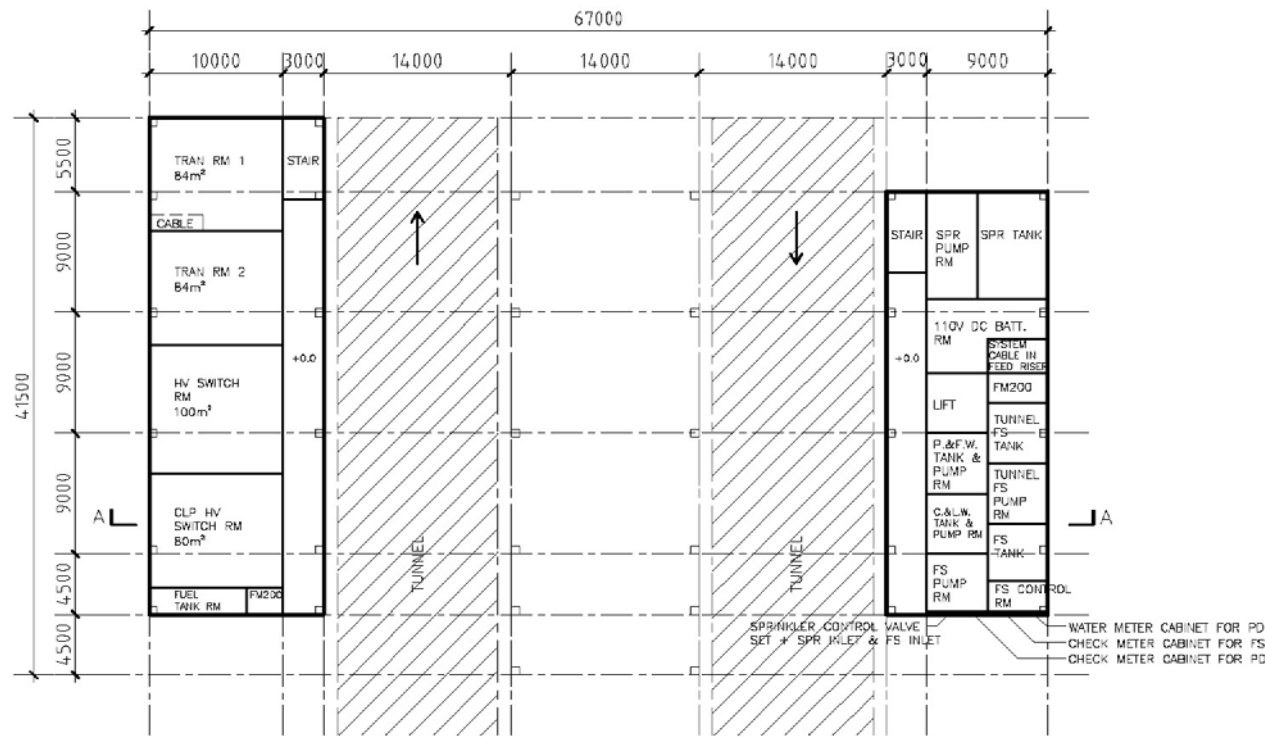
GROUND FLOOR LAYOUT PLAN (+0.0)
