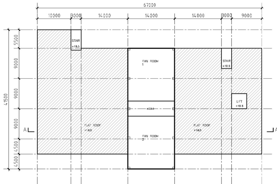
SECOND FLOOR LAYOUT PLAN (+23.5)
