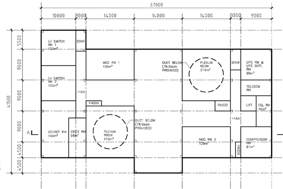
FIRST FLOOR LAYOUT PLAN (+13.5)
