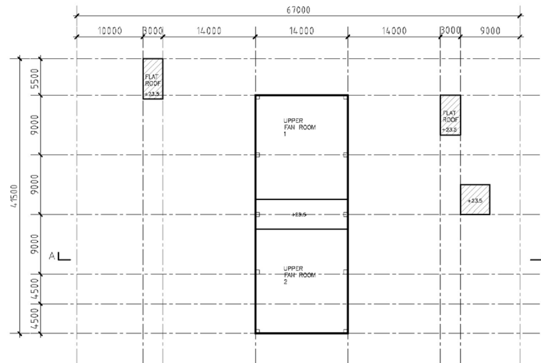
THIRD FLOOR LAYOUT PLAN (+28.5)
