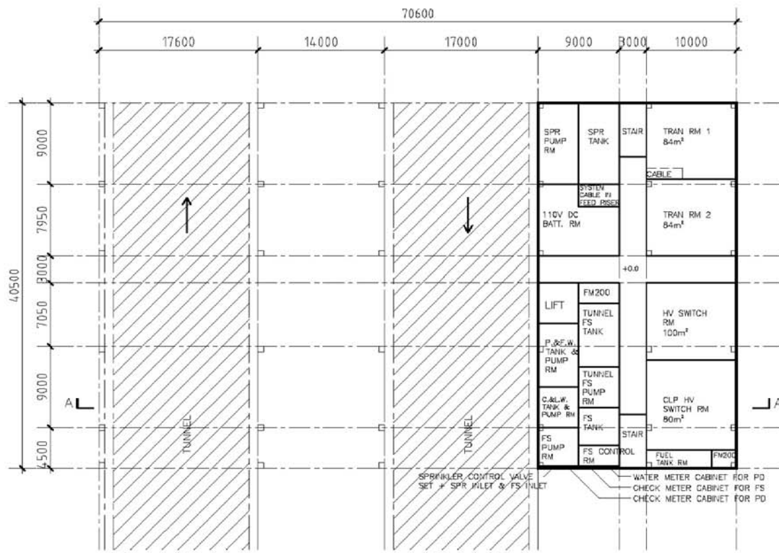
GROUND FLOOR LAYOUT PLAN
