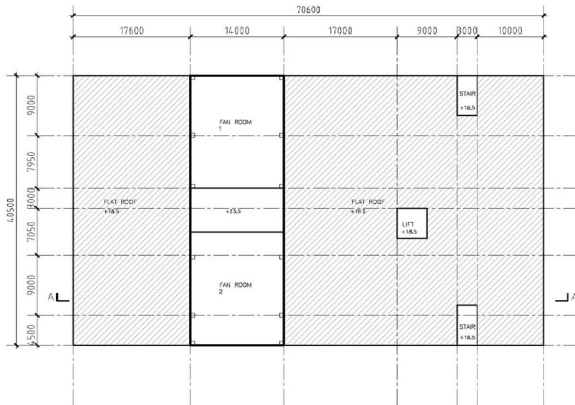
SECOND FLOOR LAYOUT PLAN
