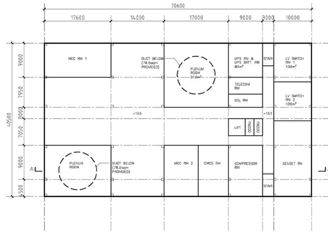
FIRST FLOOR LAYOUT PLAN
