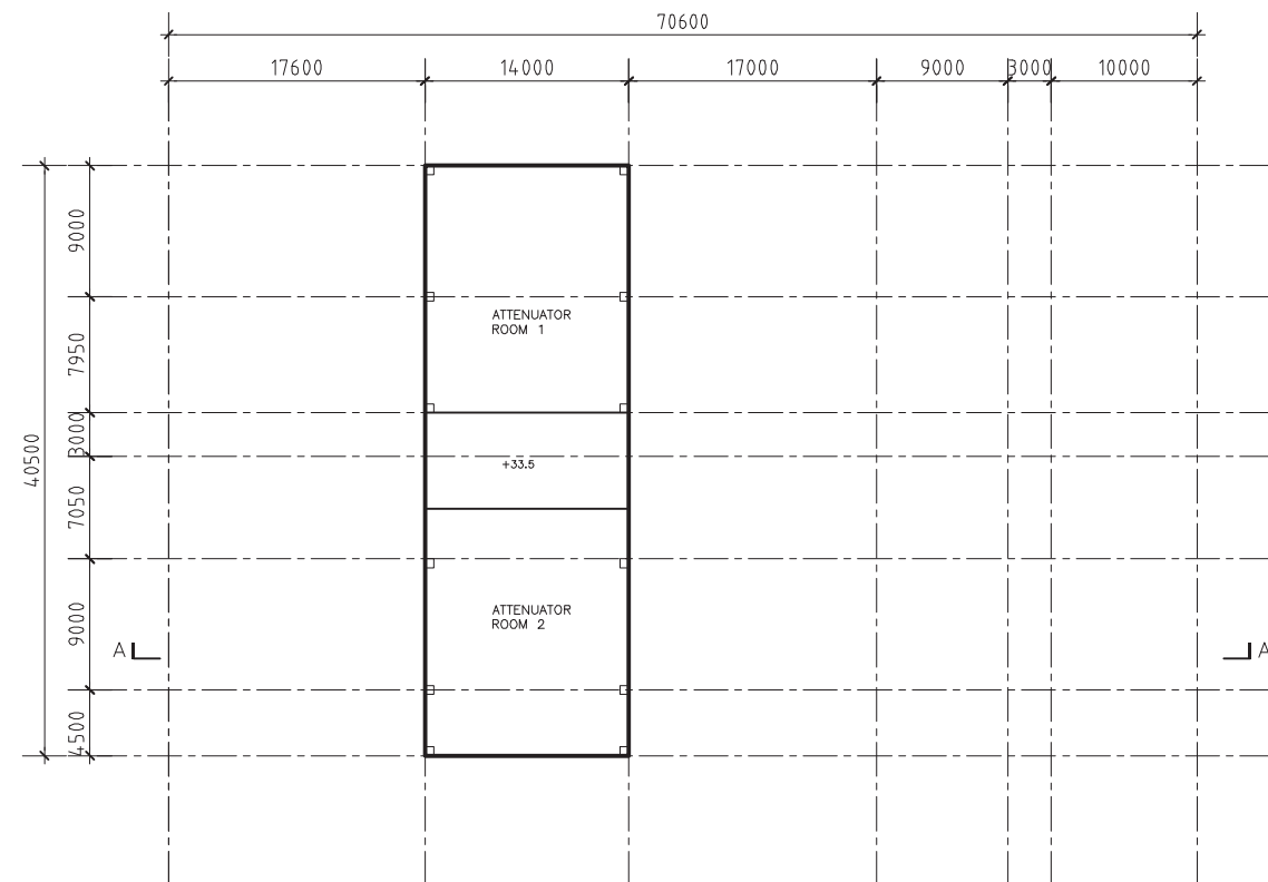
FOURTH FLOOR LAYOUT PLAN
