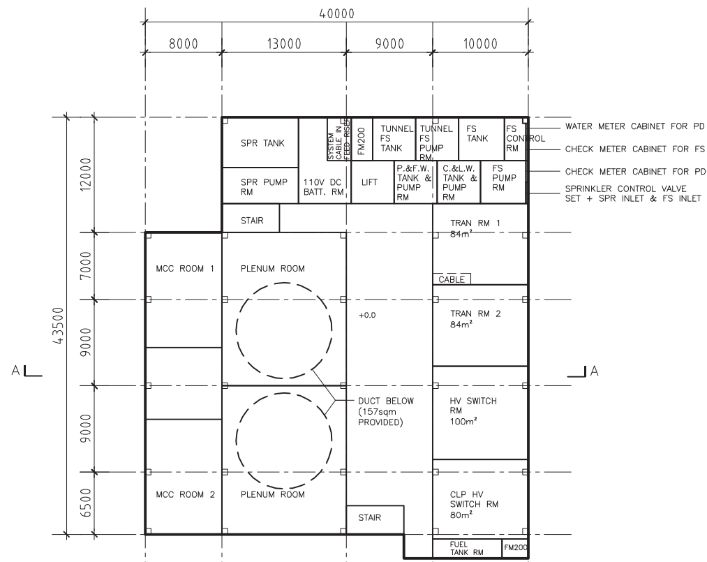
GROUND FLOOR LAYOUT PLAN (+0.0)
