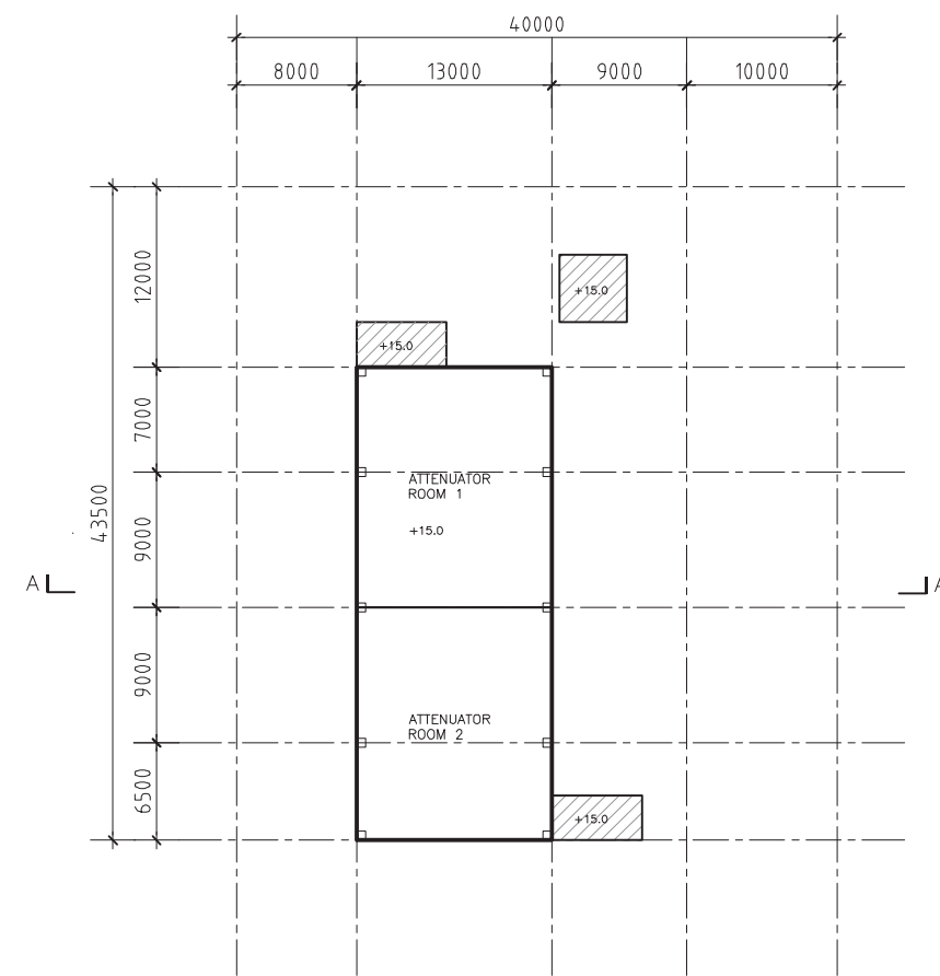
THIRD FLOOR LAYOUT PLAN (+15.0)
