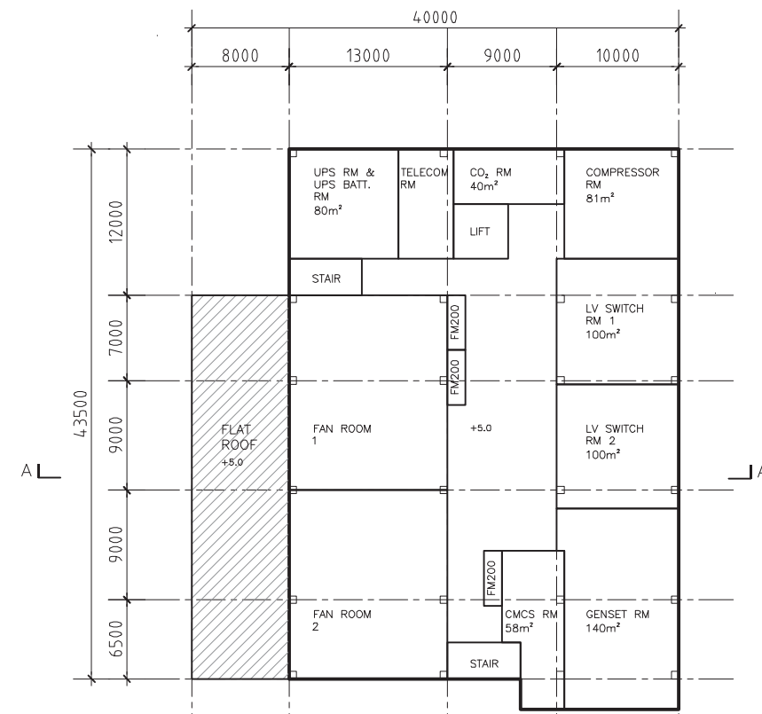
FIRST FLOOR LAYOUT PLAN (+5.0)
