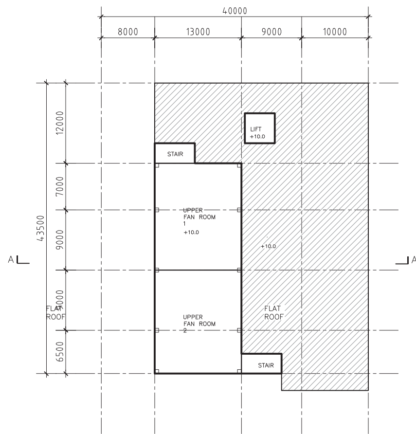
SECOND FLOOR LAYOUT PLAN (+10.0)
