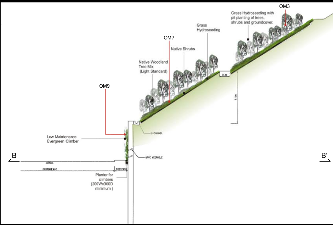
Typical Section of Slope and Retaining Wall with Mitigation Measures
