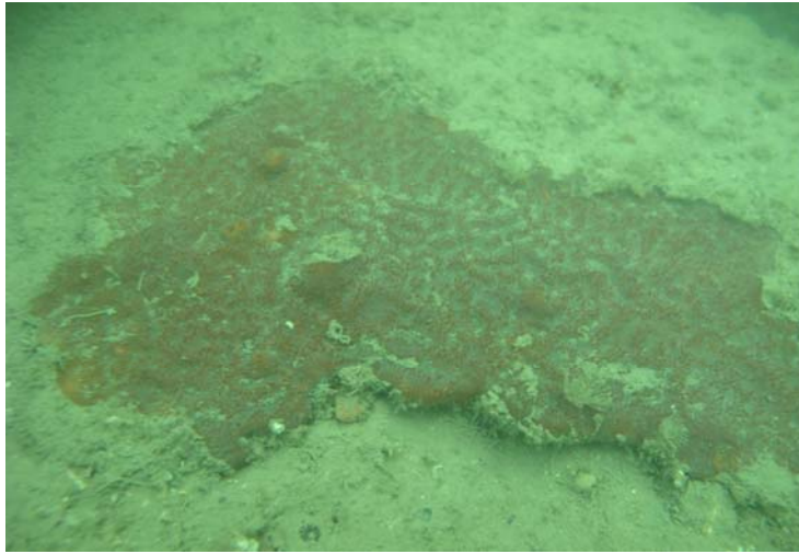
Hard coral: Coscinaraea n sp.
