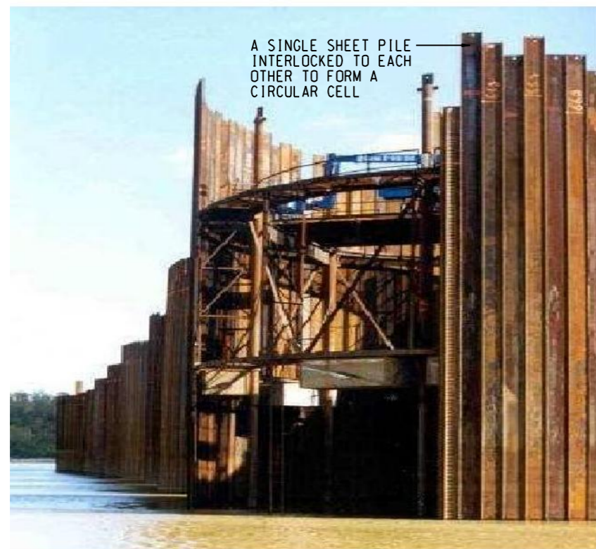
B. CIRCULAR CELL FORMED BY INTERLOCKING STRAIGHT-WEB
