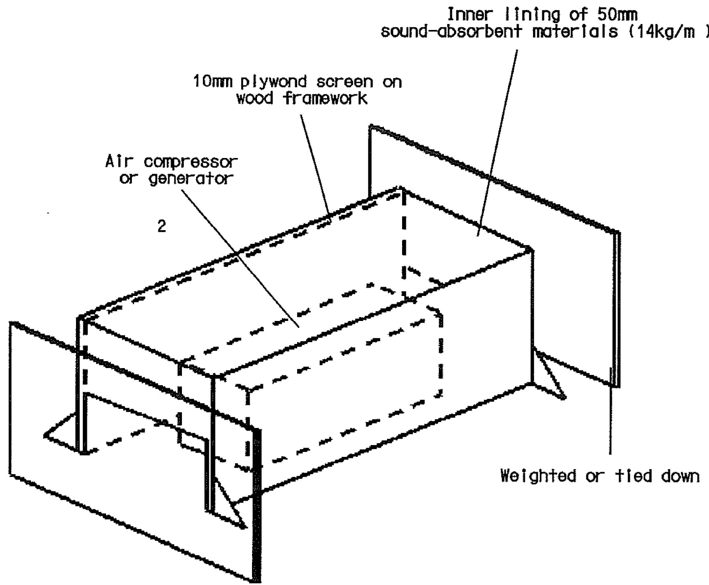
Typical Noise Enclosure for Static Plant (e.g. Air Compressors, Generators etc.) ~3-4m wall
