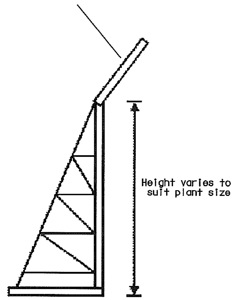
Typical Section of Temporary Movable Noise Barrier (3-5m tall)
