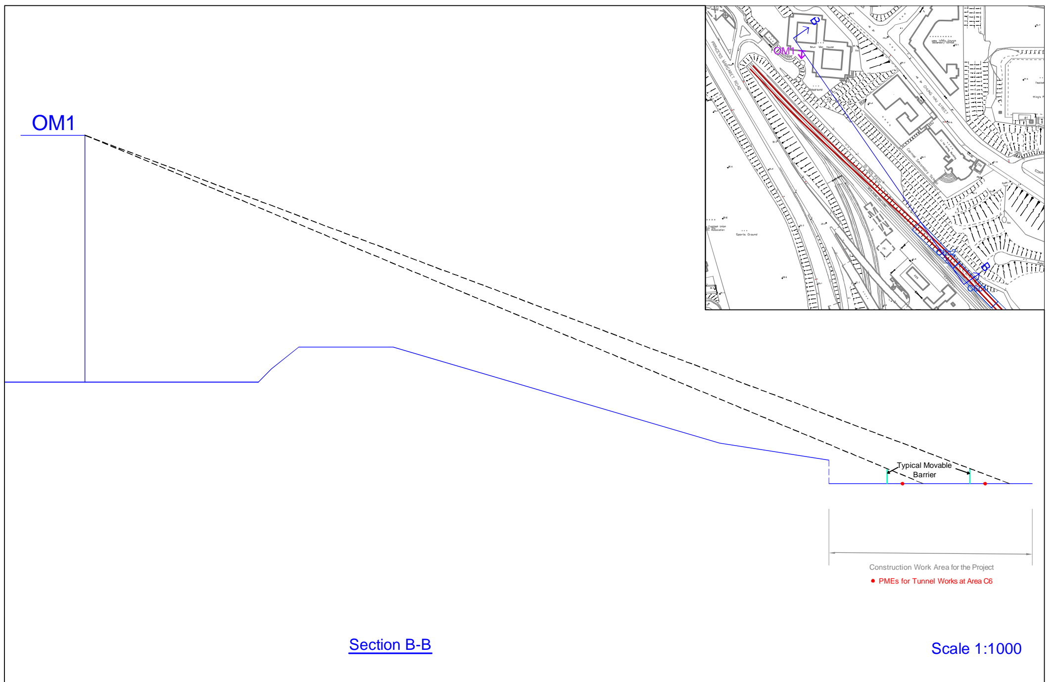
Appendix 6.11C Typical Arrangement of Moveable Noise Barriers with respect to Shun Man House (OM1).
