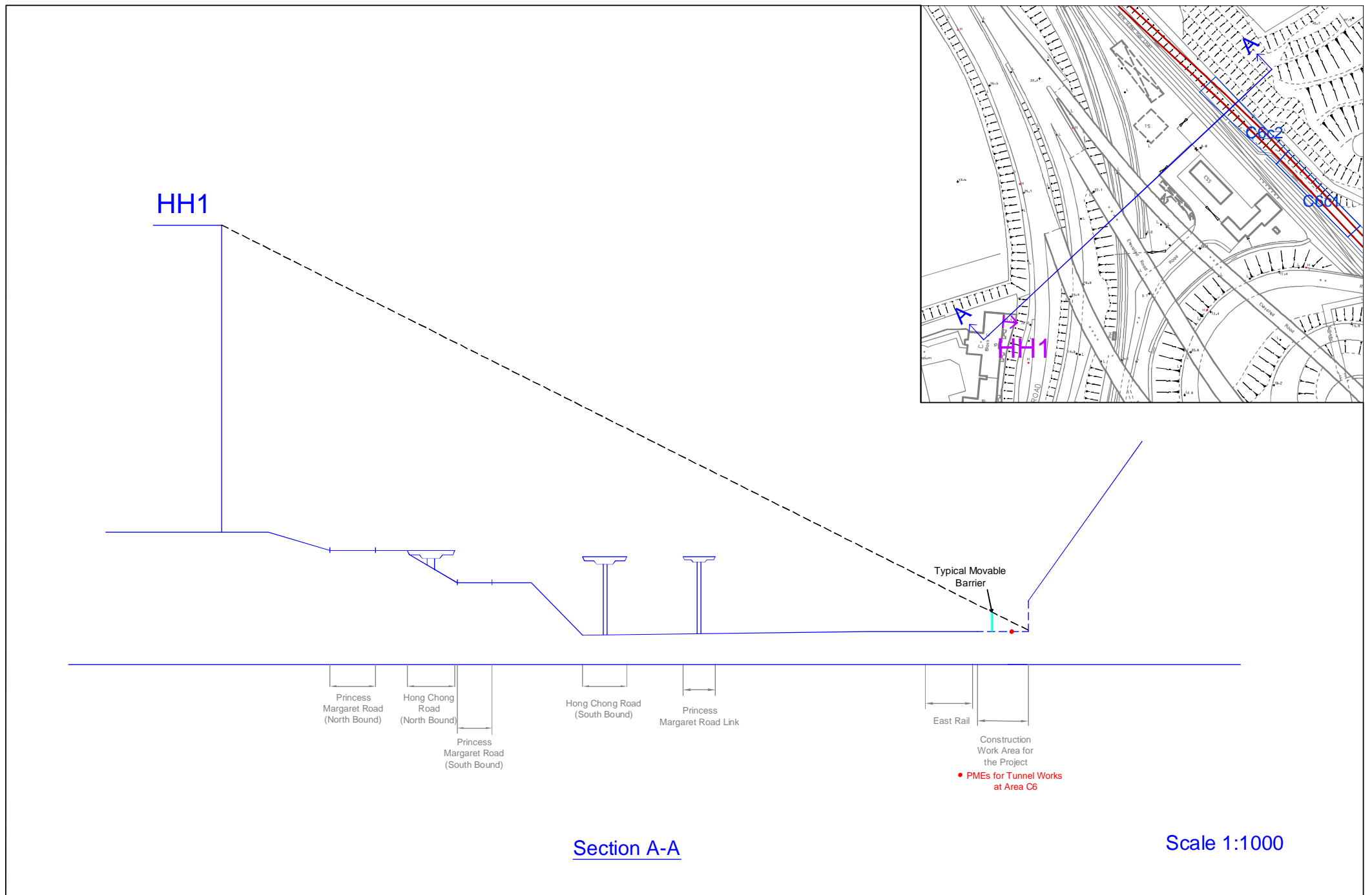
Appendix 6.11C Typical Arrangement of Moveable Noise Barriers with respect to Wylie Court (HH1).
