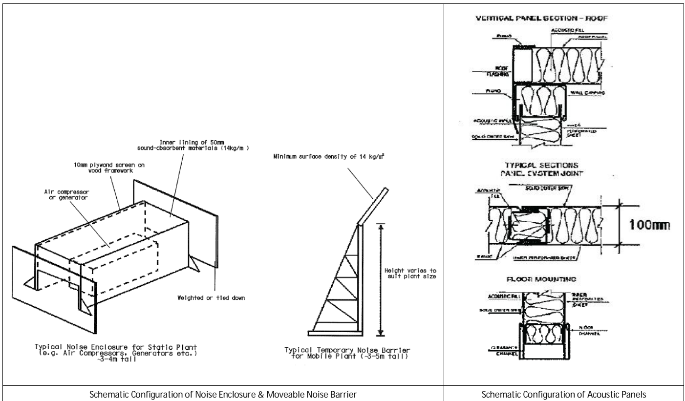
Appendix 6.11D Schematic Configuration of Noise Enclosure, Moveable Noise Barrier and Acoustic Panels.
