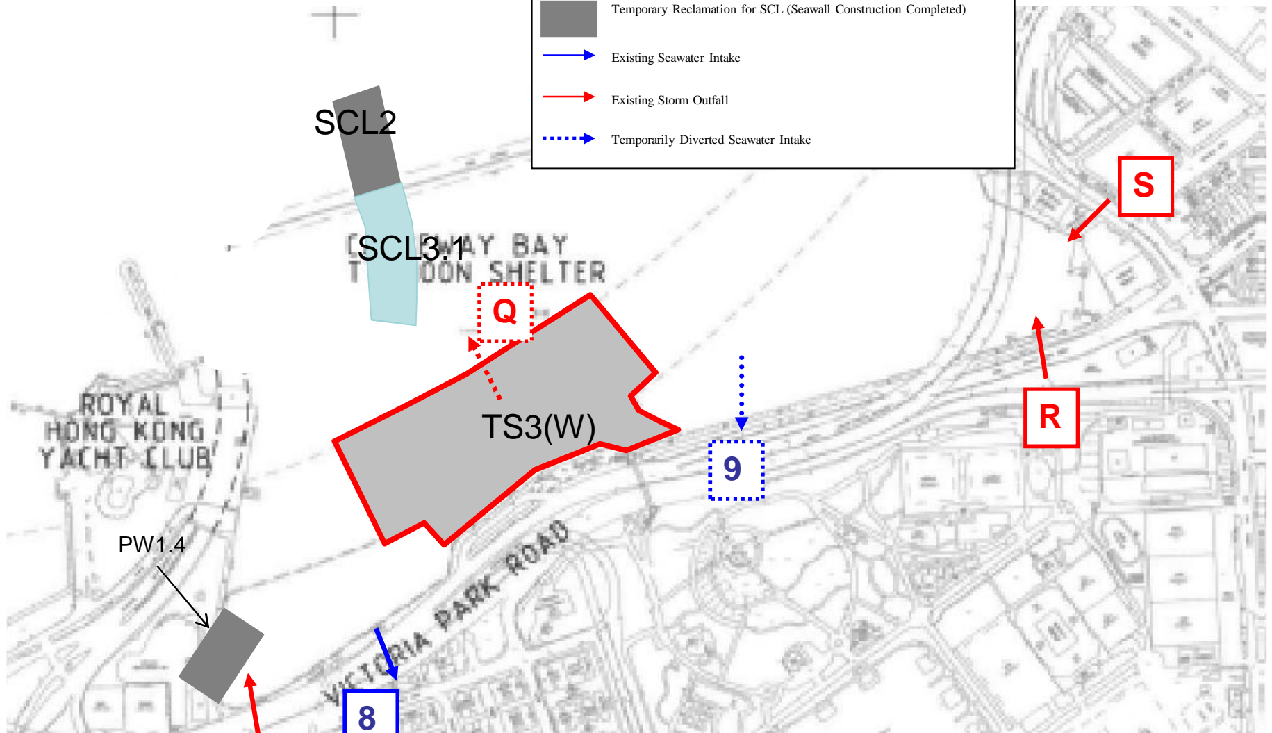
Temporary Reclamation Stages (Sheet 9 of 14)
