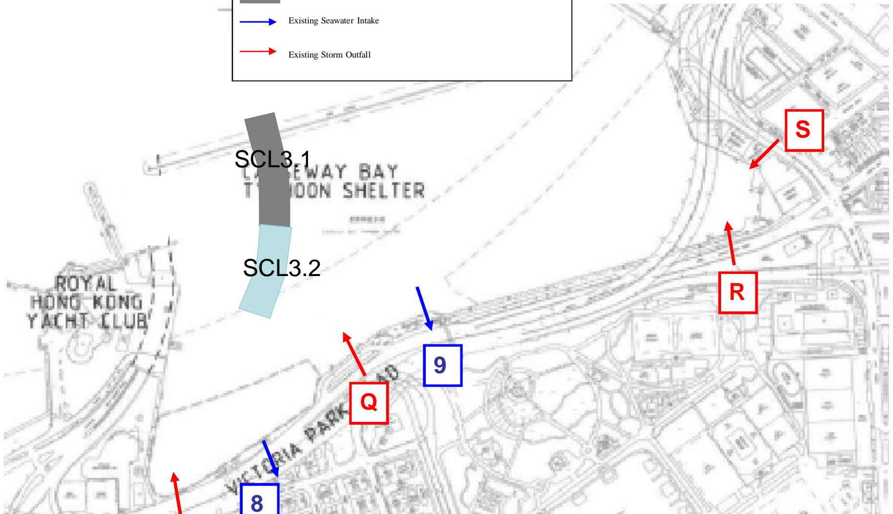
Temporary Reclamation Stages (Sheet 11 of 14)
