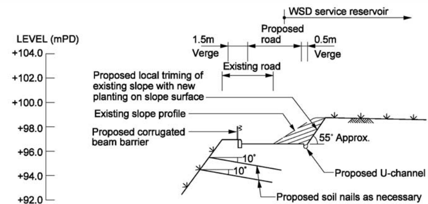
Typical Road Improvement Works at Section 4 - 4
