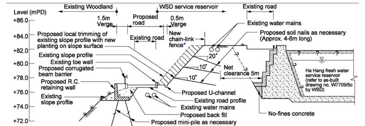
Typical Road Improvement Works at Section 3 - 3
