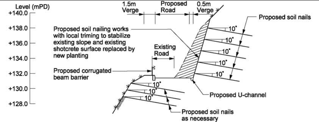
Typical Road Improvement Works at Section 5 - 5
