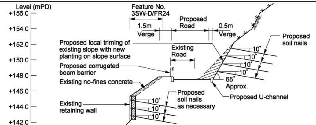
Typical Road Improvement Works at Section 6 - 6
