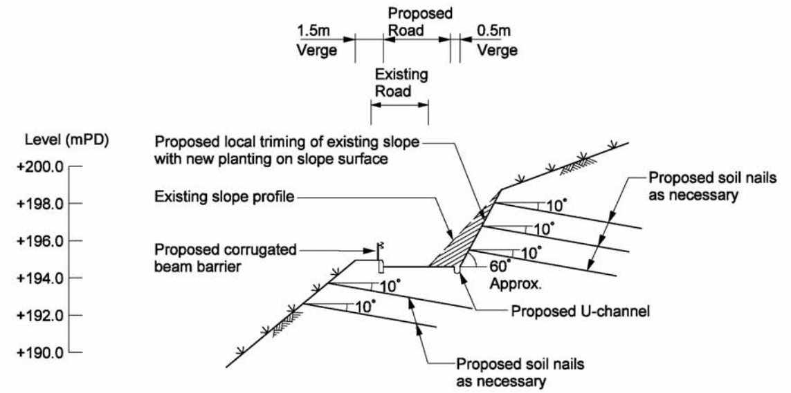
Typical Road Improvement Works at Section 7 - 7
